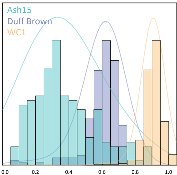
Distribution of normalized ^{238}\text{U}/^{206}\text{Pb} values
