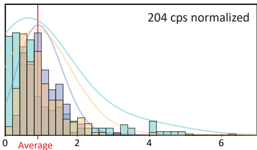
Distribution of normalized ^{238}\text{U}/^{206}\text{Pb} values
