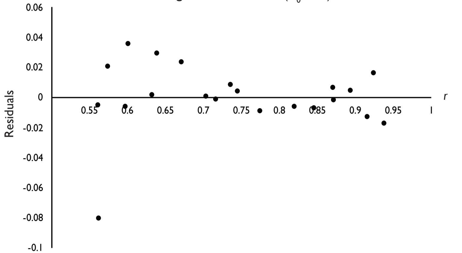
Fanning Model Residuals ( T_0 = \infty )
