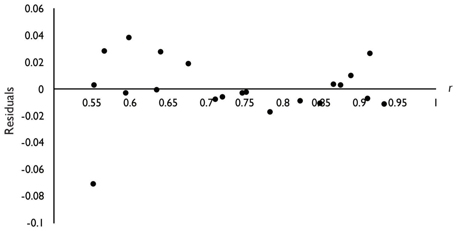
Fanning Model Residuals ( T_0 \neq \infty )
