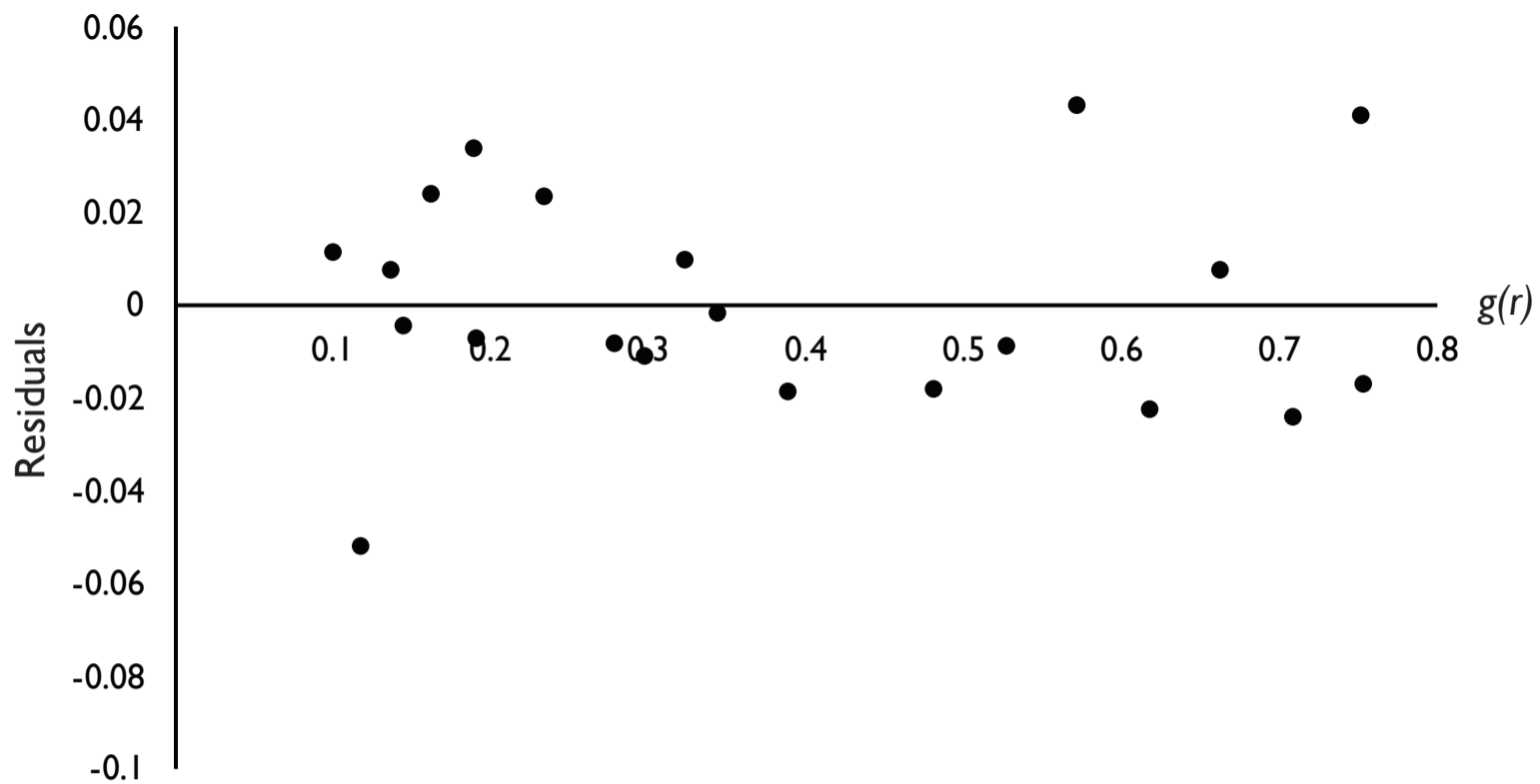
Parallel Model Residuals
