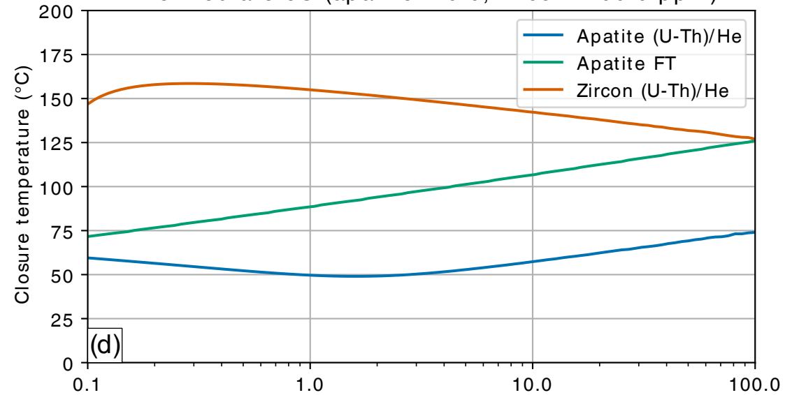
High eU (apatite=150.0, zircon=4000.0 ppm)
