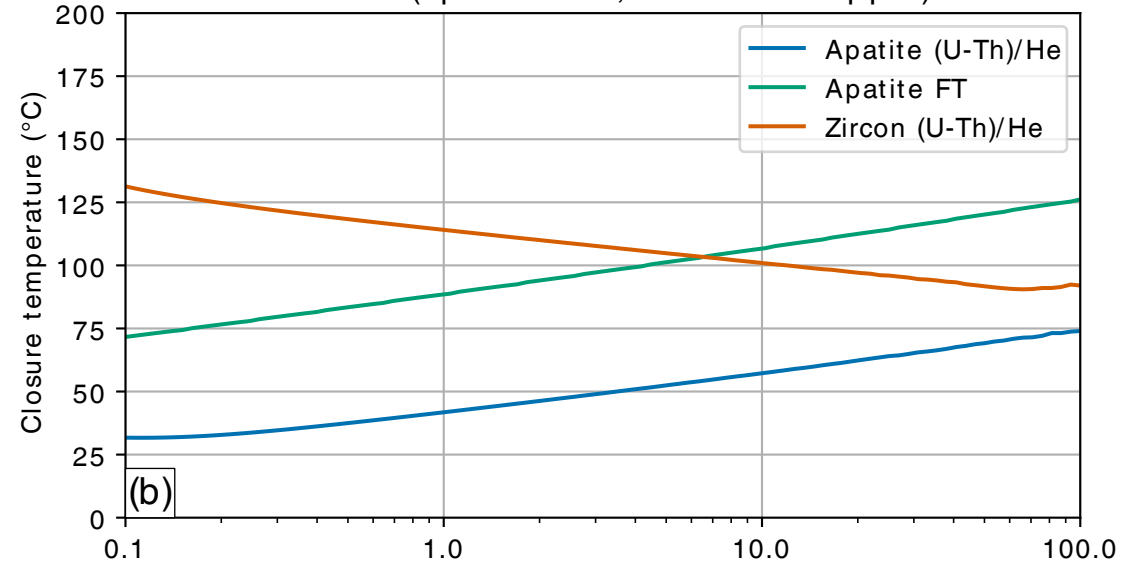
Intermediate eU (apatite=20.0, zircon=200.0 ppm)
