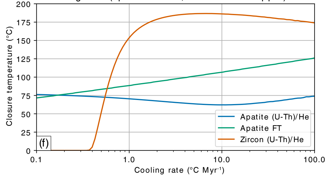
High eU (apatite=150.0, zircon=4000.0 ppm)
