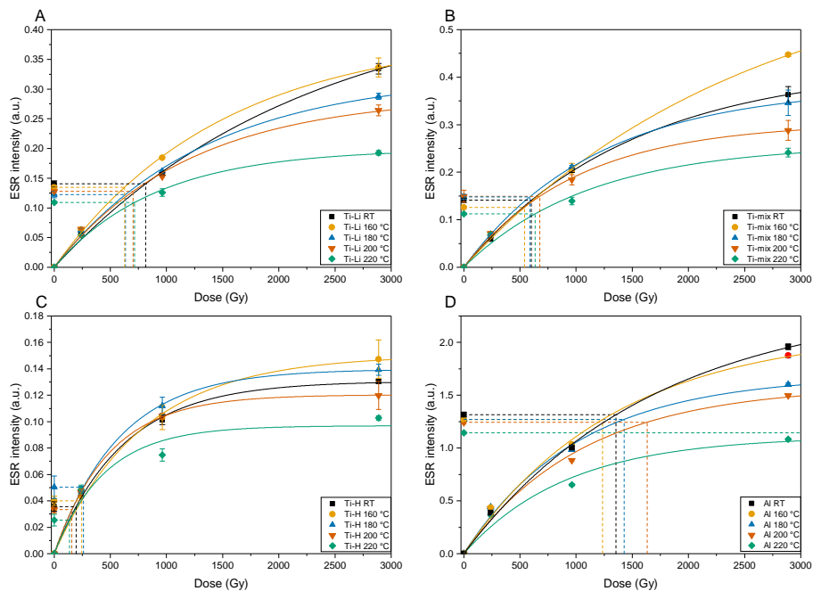
Figure S1. The DRC's for each preheat temperature (RT = room temperature = 20 °C) for each one of the ESR centres. The D_e are marked.
