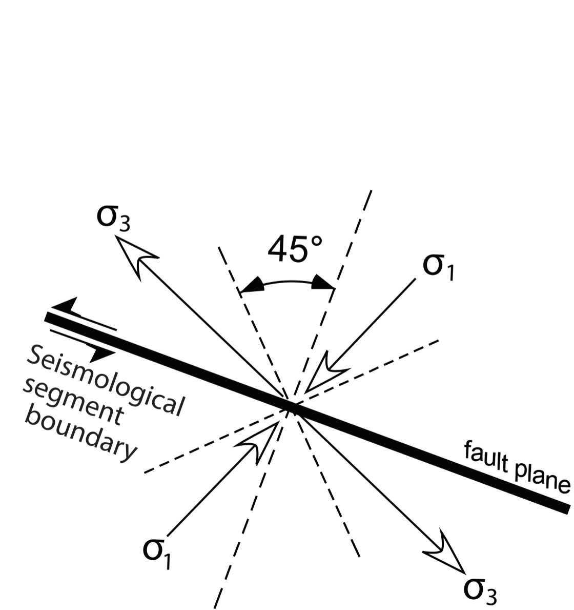
(b) Ductile failure - maximum moment
