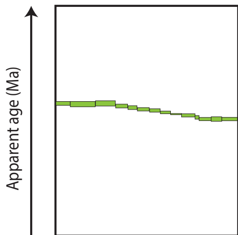
(e) Percentage released ^{39}\text{Ar}
