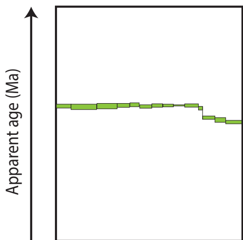
(c) Percentage released ^{39}\text{Ar}
