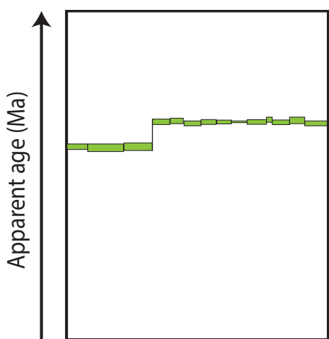
(b) Percentage released ^{39}\text{Ar}
