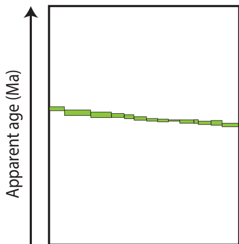
(f) Percentage released ^{39}\text{Ar}
