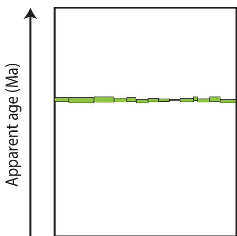
(a) Percentage released ^{39}\text{Ar}
