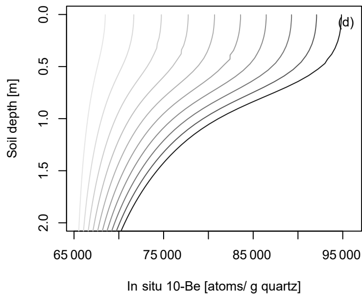
In situ ^{10}\text{Be}
