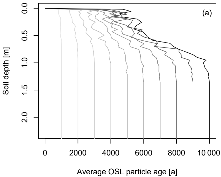
OSL particle age
