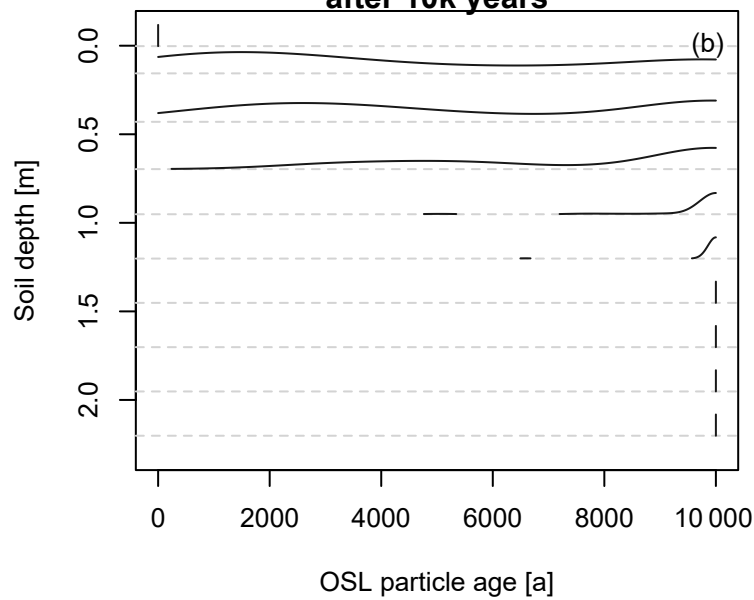
OSL particle age distributions after 10k years
