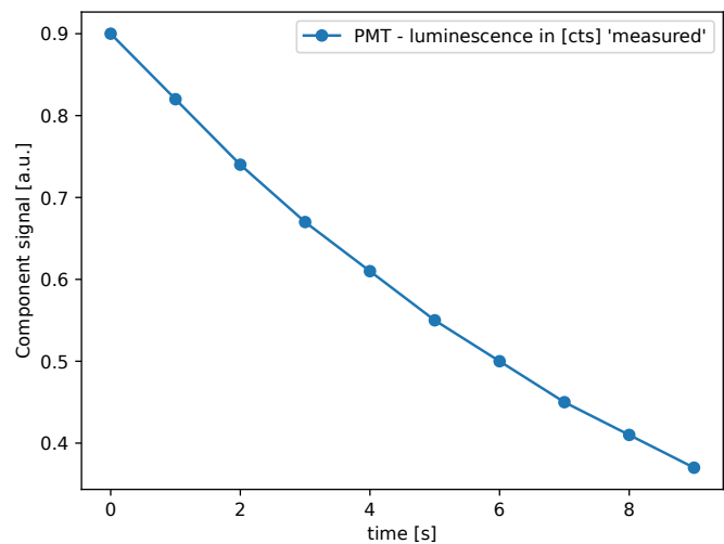
(b) LUM-21321: quartz from (-4.07, 52.41, 50.00) Testsequence.seq by DeviceEditor 2.0 GSL - standard green OSL step
