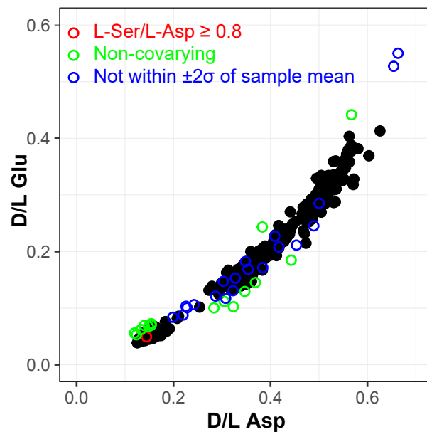
Supplementary Figure S1: Covariance of aspartic acid and glutamic acid D/L values in all subsamples prior to data screening (left), and following data rejection (right) in N. pachyderma and C. wuellerstorfi . Open symbols represent rejected subsamples.
