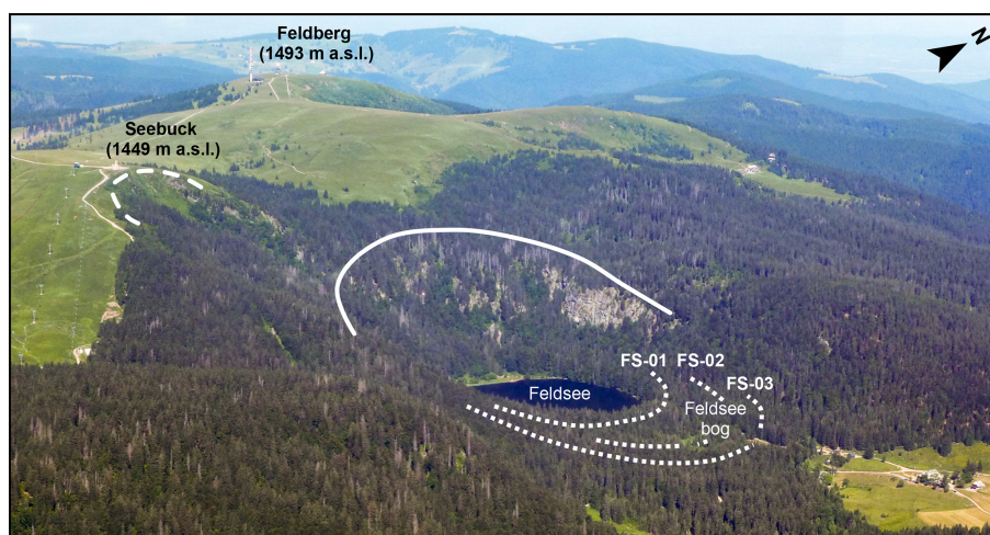
Figure 2. Oblique aerial photograph of the study site. Moraines are marked with dotted lines. The upper limit of the headwall of the Feldsee cirque is marked with a solid line. The Feldsee, a moraine-dammed lake, covers the tongue basin on the cirque floor. Note the prominent moraine at the eastern shore of the lake (position FS-01). The moraine at position FS-02 separates the Feldsee further east into two distinct basins. The bog's sediments have partly buried this moraine. To the east, the bog is bounded by the semi-circular moraine at position FS-03. Also note the initial cirque (marked with a dashed line) on the northeastern flank of Seebuck. Photo: Matthias Geyer.
