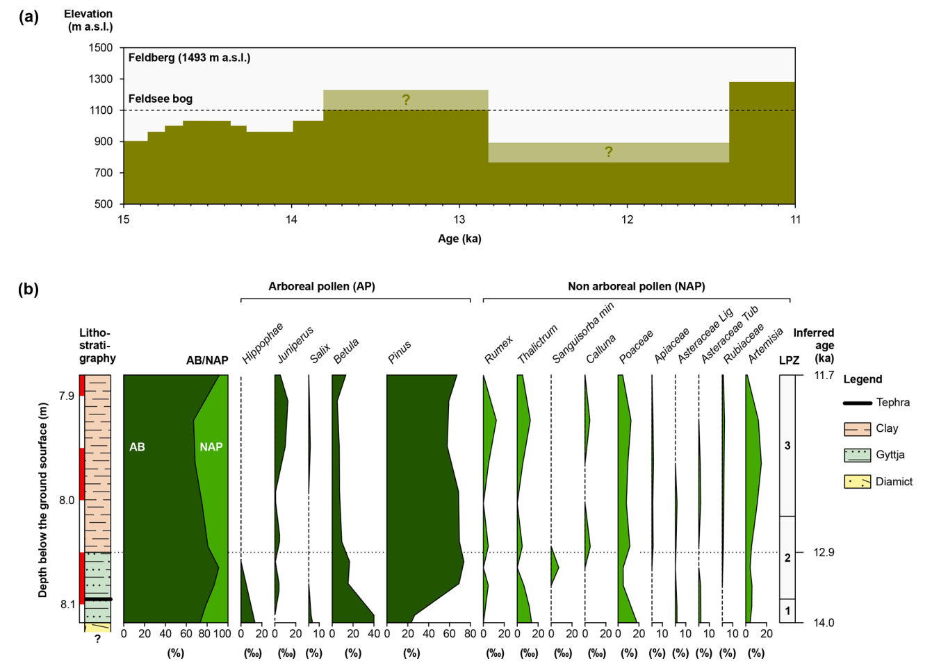
Figure 4. (a) Evolution of the timberline in the Black Forest between 15 ka and 11 ka (redrawn from Lang, 2006). (b) Lateglacial part of the sediment sequence at a coring site in the Feldsee Bog (Fig. 3b), inferred ages of the sediments, and vegetation dynamics, as documented in the pollen record. LPZ: local pollen zones. Redrawn from Lang (2005).
