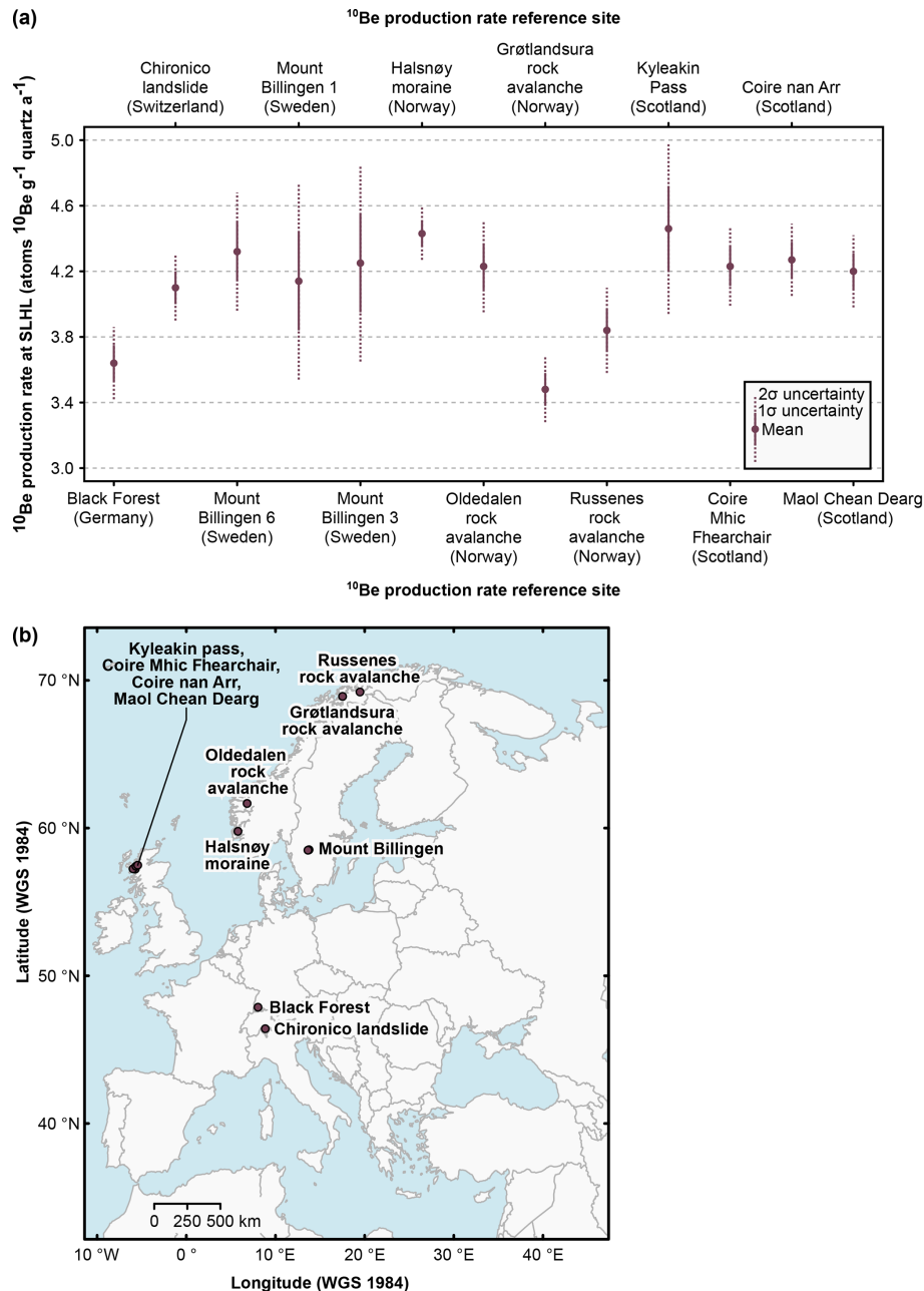
Figure 10. (a) European ^{10}\text{Be} production rates available in CREp (Martin et al., 2017). We did not include the Rannoch Moor ^{10}\text{Be} production rate in this compilation, as this production rate is not commonly accepted (cf. Lowe et al., 2019, and references therein). (b) Map of the calibration sites mentioned in panel (a).
