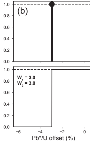
Constant Pb loss
