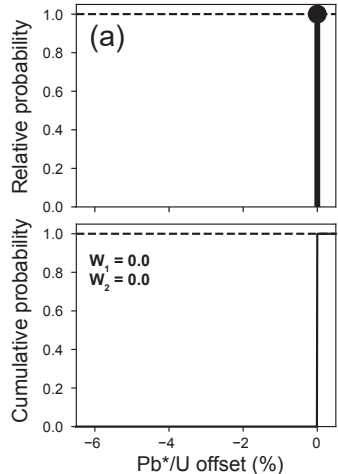
No Pb loss
