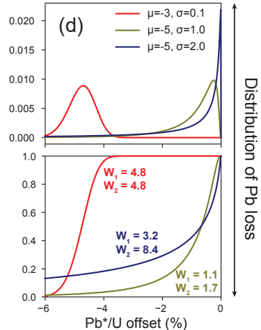
Continuous Pb loss
