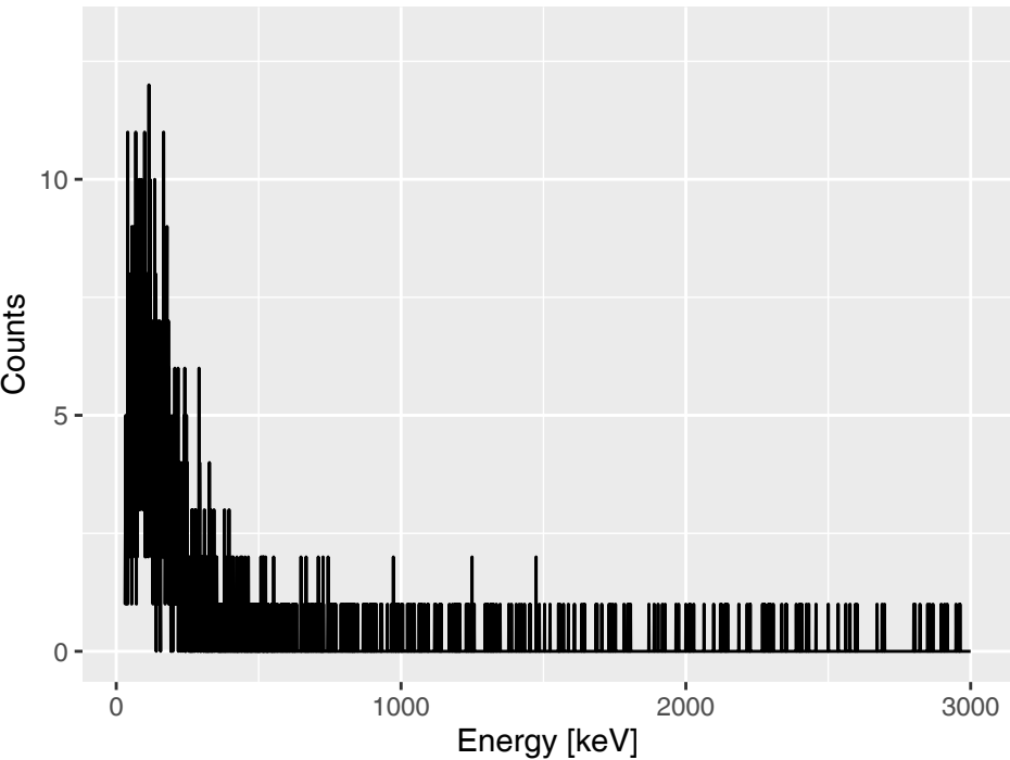
Background measurement GR1 | duration: 18 060 s
