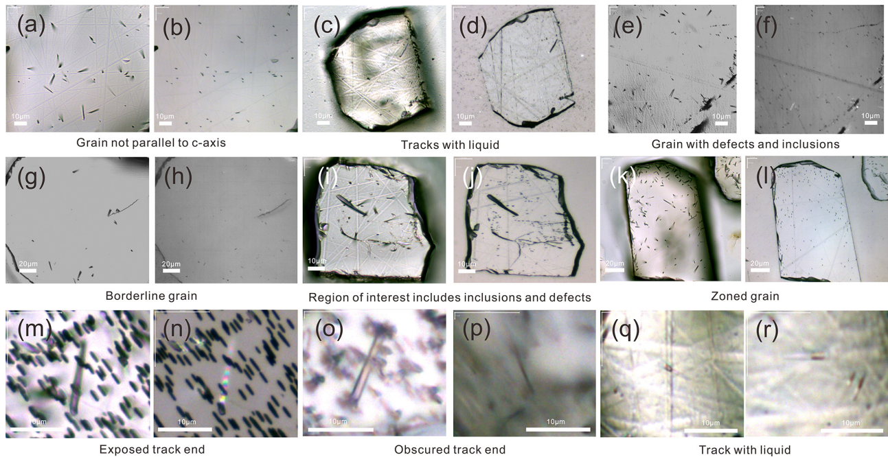
Figure 1. Examples of grains and tracks that could cause erroneous grain and region of interest selection or invalid confined track length measurement for fission-track analyses. (a) A grain not parallel to the c axis appears to be suitable in transmitted light, (b) but varying etch pit orientations clearly show that the grain is not parallel to the c axis in reflected light. (c, d) Transmitted and reflected light images showing how a dirty grain surface with liquids in tracks can impair track recognition. (e, f) Transmitted and reflected light images of a grain showing an excess of non-track features such as defects and inclusions that are difficult to distinguish from actual tracks. (g, h) Transmitted and reflected light images of a grain with a low and uneven track density, suggesting the possible presence of zoning that would need to be accounted for. (i, j) Transmitted and reflected light images of a grain showing large defects and inclusions occupying space and obscuring fission tracks, resulting in underestimation of the fission-track density if these features are included in the region of interest. (k, l) Transmitted and reflected light images of a zoned grain, for which different placements of the region of interest and location of ablation point(s) may yield divergent ages. (m, n) Transmitted and reflected light images of a would-be confined track, where the reflected light image shows that one tip may be exposed to the surface. (o, p) Confined tracks may also be rendered invalid for measurement by obscuring features (q, r) or partial fluid fillings.
