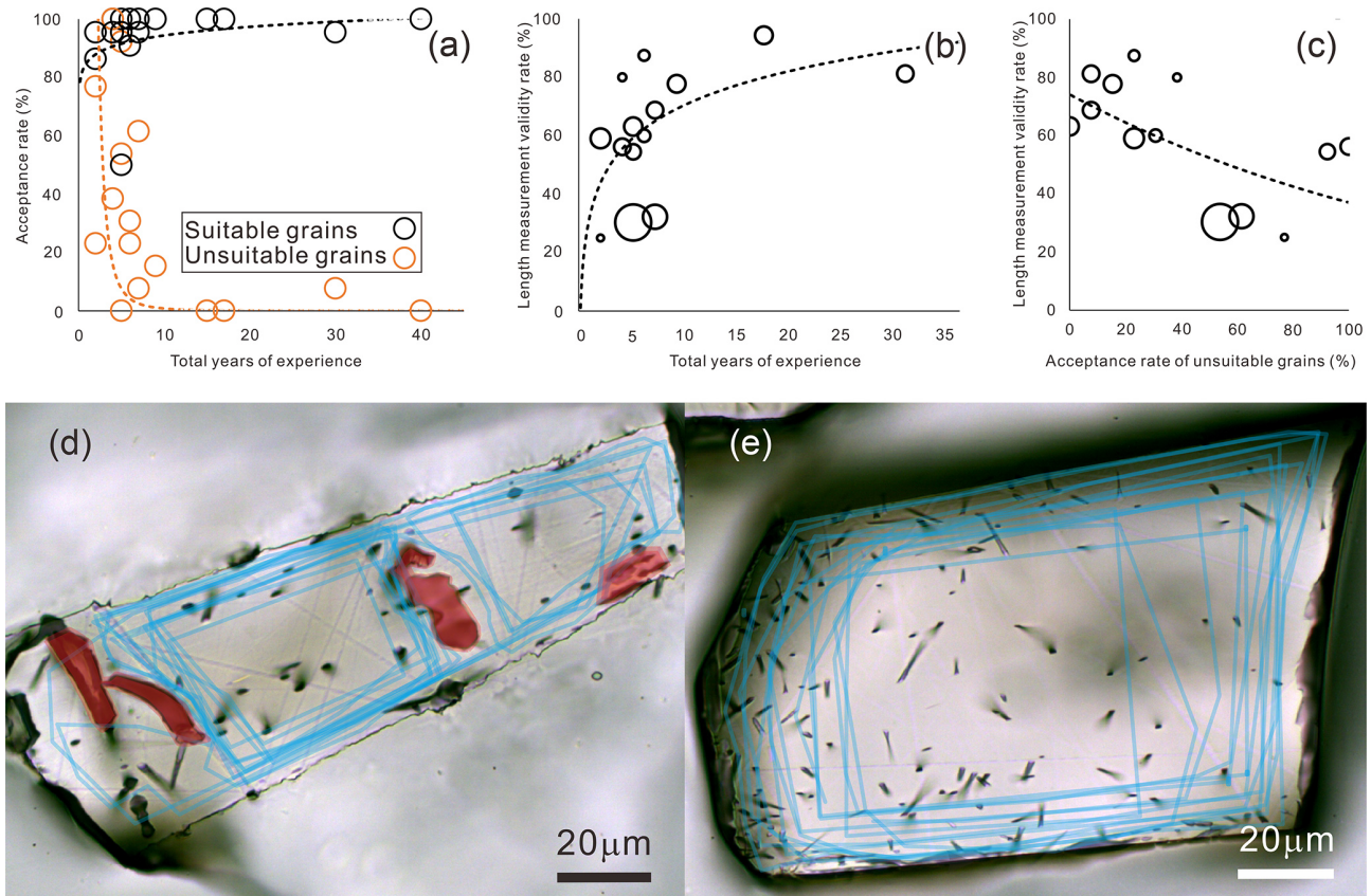
Figure 4. (a) Correlation of years of fission-track experience against acceptance percentage of suitable and unsuitable grains for density measurement and (b) confined track length measurement validity percentage. (c) The confined track length measurement validity percentage against the acceptance percentage of unsuitable grains. The sizes of the circles in (b) and (c) reflect the number of confined track length measurements. (d) Participant sections of the region of interest are juxtaposed in a defect- and/or inclusion-rich grain and (e) a zoned grain.
