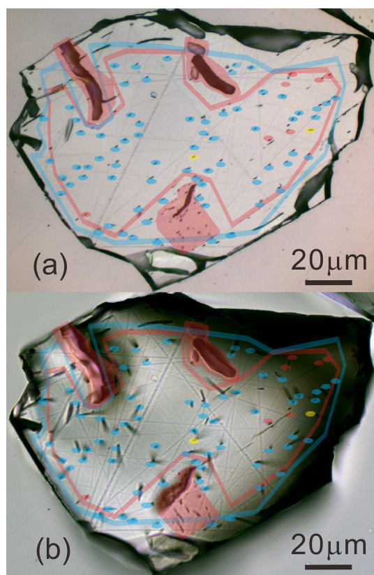
Figure 5. Transmitted and reflected light images of Grain 07 (a, b) with the analysis of one participant (blue) and a reviewer's proposed correction for inclusion (red) and exclusion of tracks (yellow).
