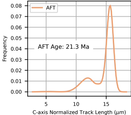
c) Track Length Distribution
