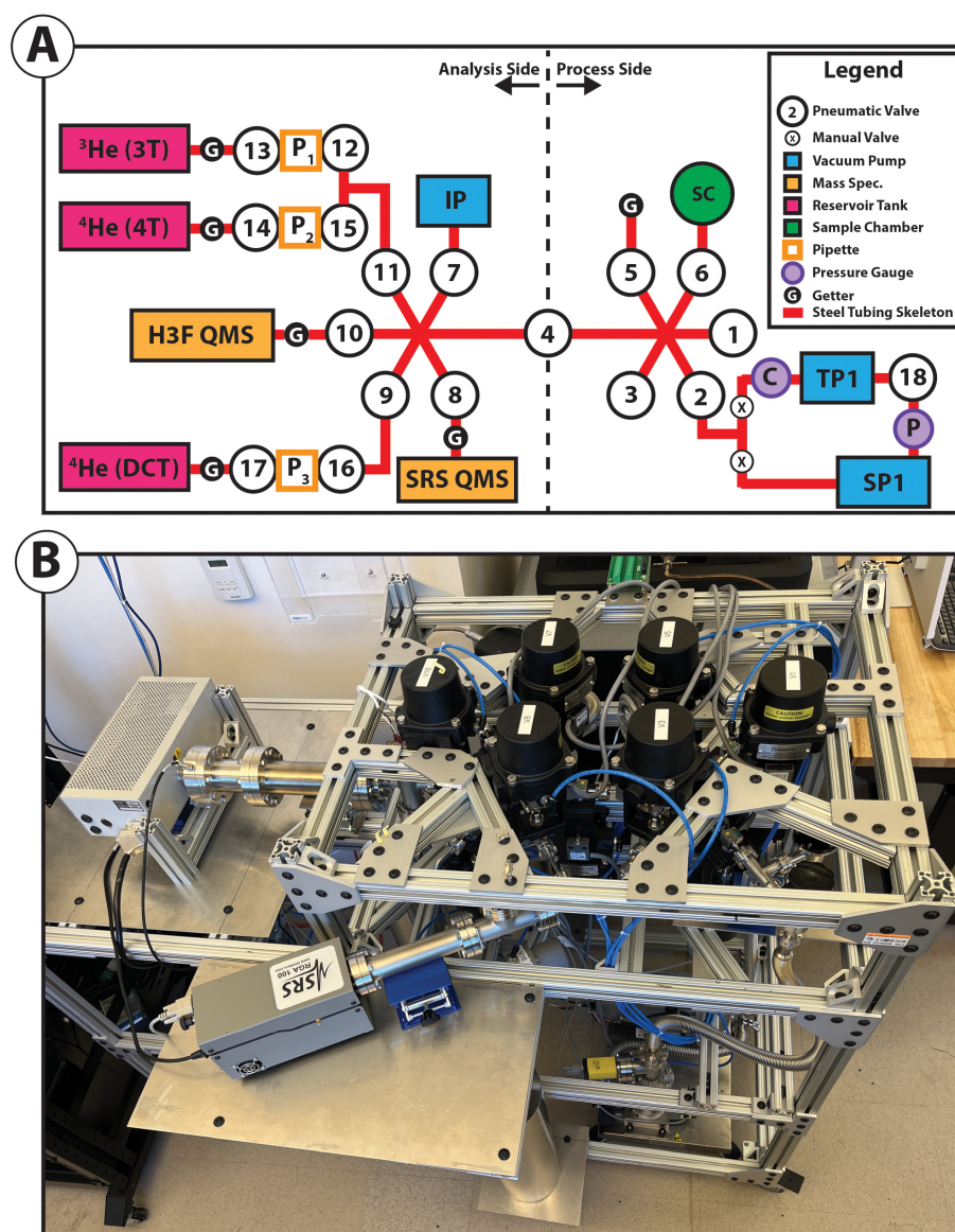
Figure 1. (A) Schematic diagram of the Jimbochron highlighting key components and connections. The line is conceptually divided into a “Process Side” which is exposed to relatively high pressures of atmospheric gas during sample exchange, and the “Analysis Side” which only regularly sees gas that has been gettered and cleaned. The three vacuum pumps (in blue) are the Ion Pump (IP), Turbo Pump (TP), and Scroll Pump (SP). The three reservoir tanks (in pink) are the 3T tank that contains ^3\text{He} , and the 4T tank and DCT (depletion-correction tank) that contain ^4\text{He} . The tanks each have a getter and are attached to three separate pipettes labeled P1, P2, and P3. The two quadrupole mass spectrometers (QMS, solid orange boxes) are the Hiden 3F ® (labelled H3F) and the Stanford Research Systems RGA100 ® (labelled SRS). The purple circles are the Pirani (P) and Cold Cathode (C) pressure gauges. (B) Picture of the Jimbochron in a similar orientation to the schematic diagram in (A). Note many of the valves are mounted with the actuators facing down and not visible in the picture.
