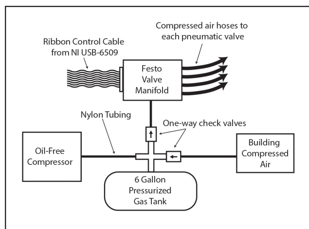
Figure 2. Schematic diagram of the compressed air backup system. A 6-gallon stainless-steel tank is connected through a tee-connector to a pressure-activated oil-free compressor, the building compressed air supply, and the Festo® valve manifold. One-way check valves ensure that if building air pressure is lost, the tank and compressor volumes will maintain their air pressure (direction of allowed flow shown by the arrows).
