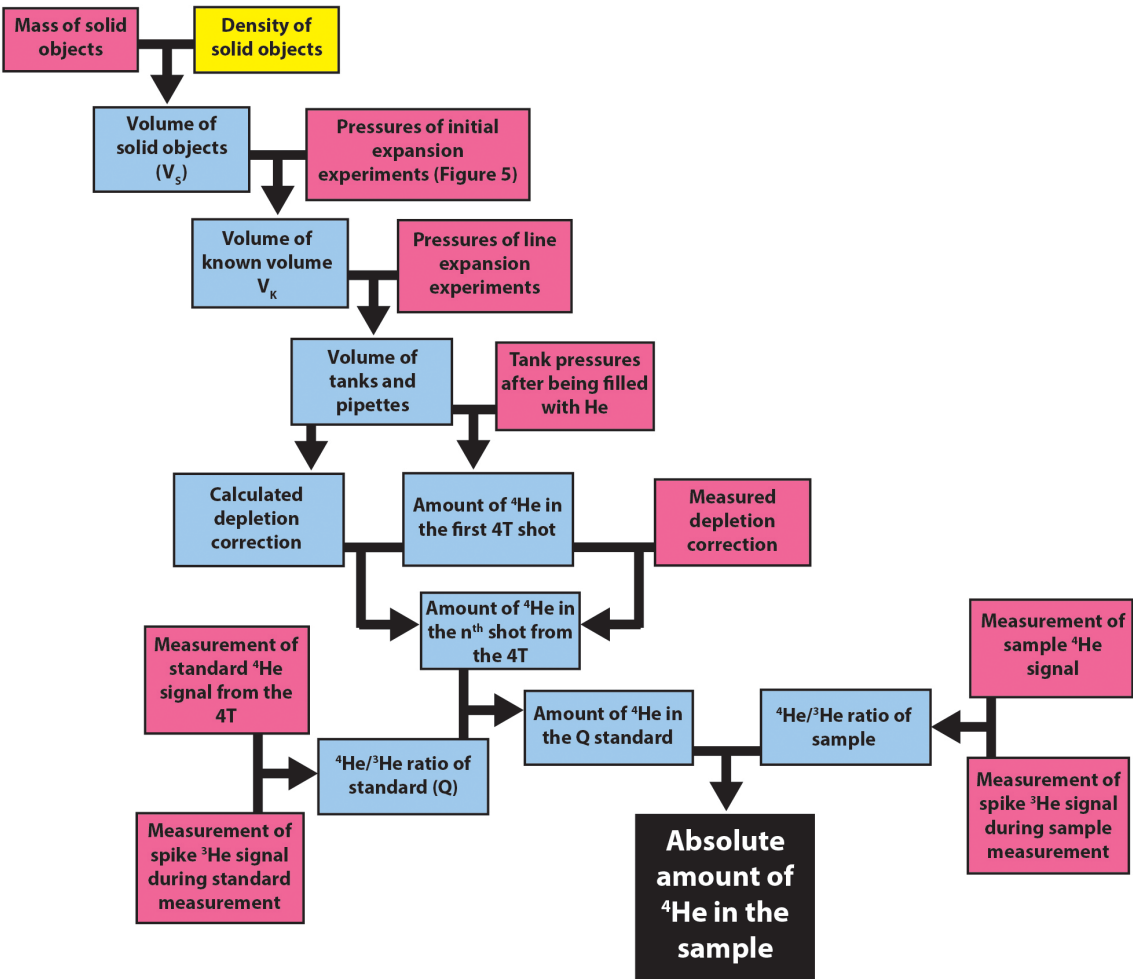
Figure 4. Flow chart showing how the absolute amount and uncertainty of ^4\text{He} in a sample (black box) are determined. The coloured boxes are measured values (pink), calculated values (blue), and values obtained from the literature (yellow). The black lines and arrows represent calculations where uncertainties are propagated.
