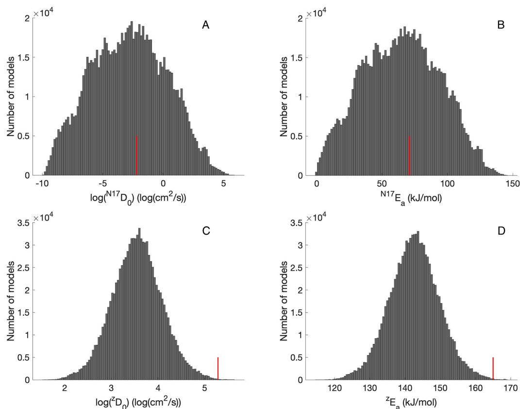
Figure 2. The sampled marginal posterior distributions for the four diffusion parameters representing the two hypothetical crystals. (A) and (B) are the frequency factor ( N^{17}D_0 ) and activation energy ( N^{17}E_a ), respectively, for an extremely damaged crystal. (C) and (D) are the frequency factor ( ^2D_0 ) and activation energy ( ^2E_a ), respectively, for a minimally damaged crystal. The red lines show the values of these parameters used by Guenthner et al. (2013).
