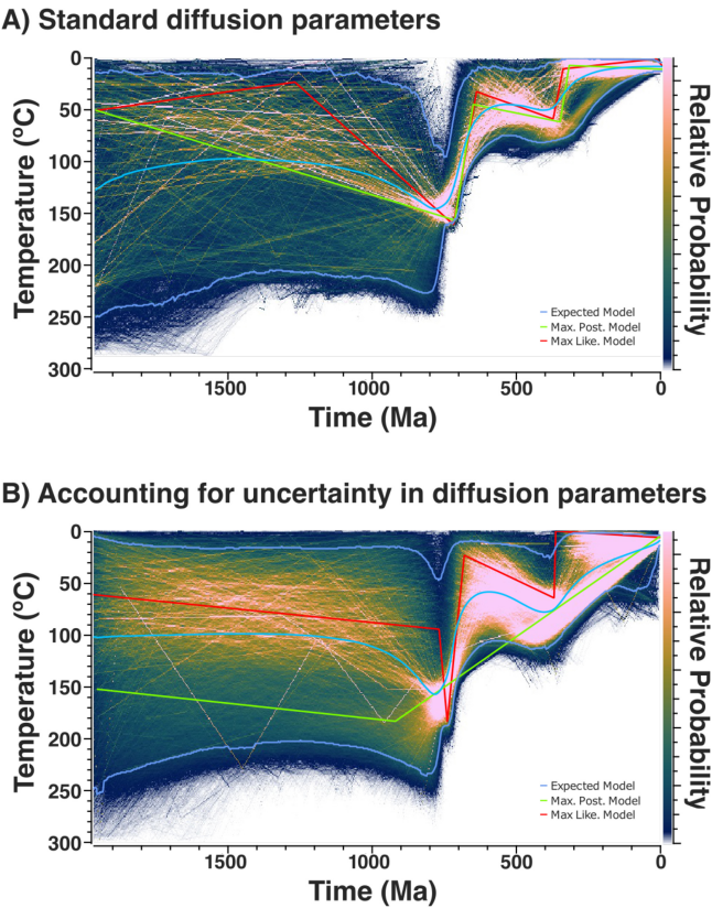
Figure 5. Thermal histories inferred using QTQt with (A) the Guenthner et al. (2013) diffusion parameters and (B) resampling of the 4 diffusion kinetics parameters. The dataset used for this analysis is reported in McDannell et al. (2022). The resampling leads to a wider distribution of possible thermal histories, wider credible intervals, and also identifies 2 different forms, or modes in the posterior distribution (as seen by the Max Posterior and Max. Likelihood models). Note in this case, the expected, or average, model falls between the two modes and so makes less good predictions relative to the other two models (see log-likelihoods in Table 3).
