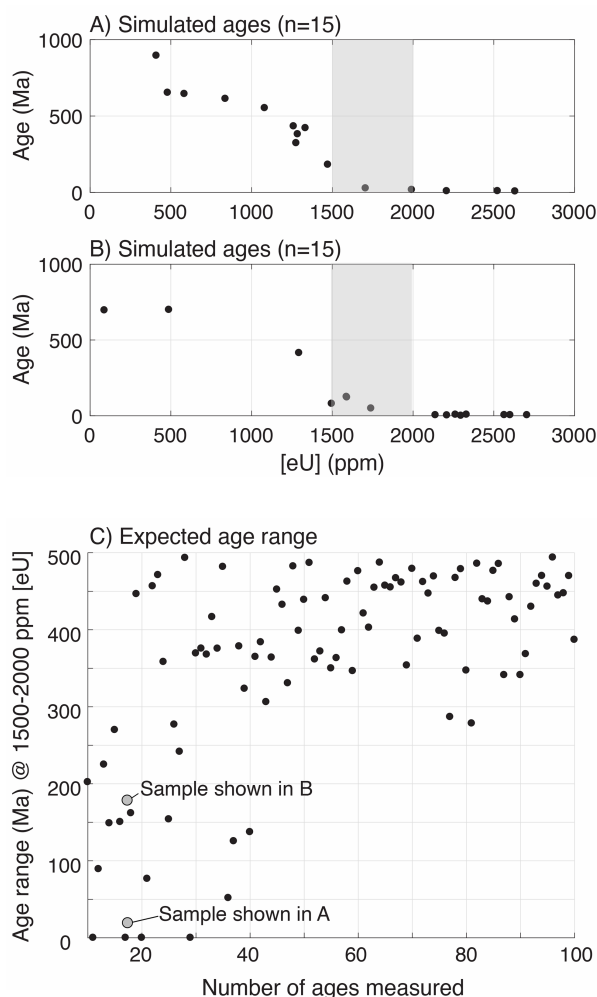
Figure 6. Model realizations and expected ranges of ages. (A, B) random samples are drawn from the probability distribution in Fig. 4 to highlight the sorts of datasets that are expected given the typical number of ages measured on a single sample. The simulated ages are different between the two realizations of a typical dataset. The gray regions show the [eU] range inspected in panel (C). (C) Many ages need to be sampled in order to accurately capture the spread in ages over a specific [eU] bin.
