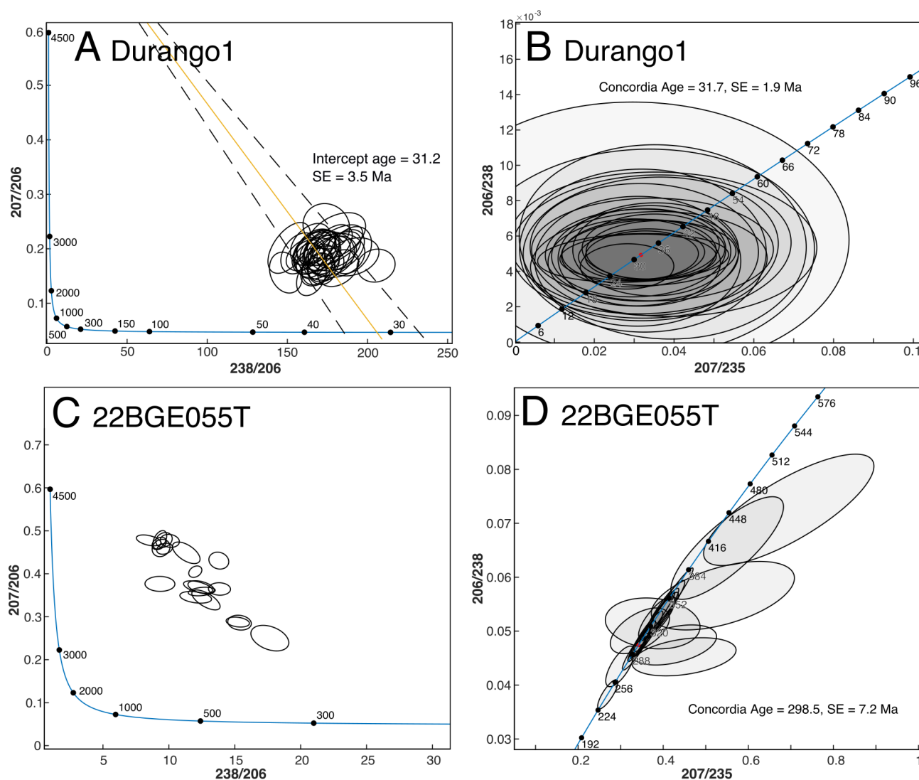
Figure 4. Apatite U-Pb data for Durango1 and 22BGE055T. (A, C) Tera-Wasserburg diagram. (B, D) Concordia diagram with derived lower intercept, concordia age and standard error (SE). Note that single grain data of 22BGE055T does not define a statistically significant linear trend, preventing the derivation of a meaningful lower intercept in the Tera-Wasserburg diagram.
