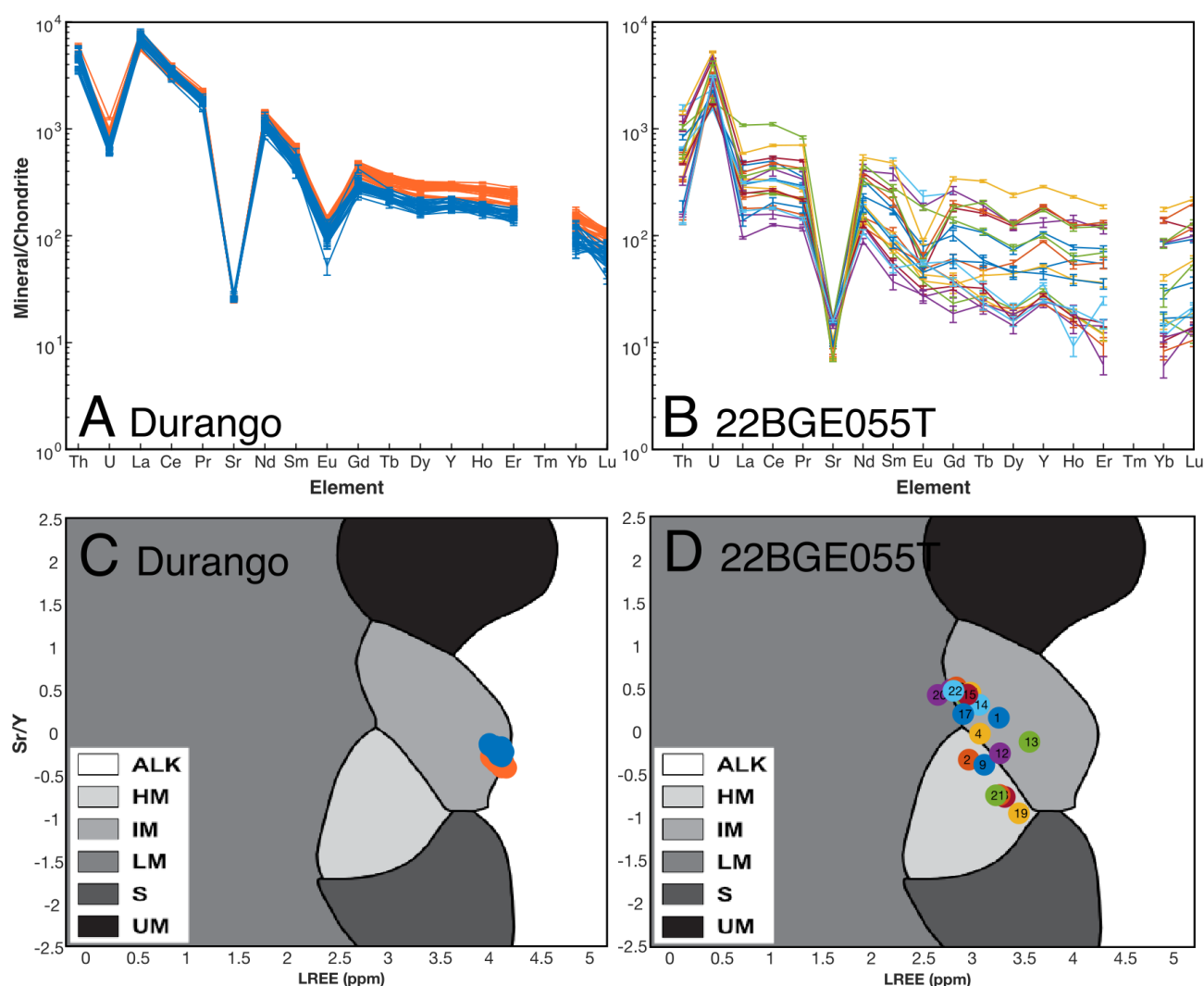
Figure 3. (A, B) Chondrite-normalised rare earth element (REE) plus U, Th and Sr multi-element plot (spider diagram) of Durango apatite (red – Durango1, blue – Durango2) and sample 22BGE055T. Gaps represent non-analysed elements. (C, D) Sr/Y vs. \sum LREE biplot of Durango apatite (red – Durango1, blue – Durango2) and 22BGE055T trace element results. Background grey colours represent the classification proposed O’Sullivan et al. (2020): ALK – alkali-rich igneous, HM – partial-melts/leucosomes/high-grade metamorphic, IM – mafic I-type granitoids and mafic igneous, LM – low- and medium-grade metamorphic and metasomatic, S – S-type granitoids and high-aluminum saturation index felsic I-types, UM – ultramafic rocks including carbonatites, lherzolites and pyroxenites.
