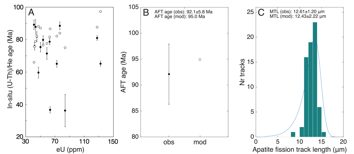
Figure 8. Observed (obs) vs. modelled (mod) thermochronological data (black dots vs. circles) of sample 22BGE055T and the best fit t – T -path that fit most input data simultaneously (black t – T -path in Fig. 7).
