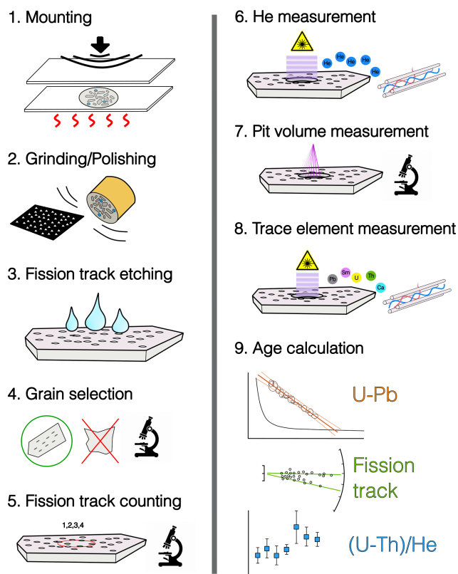
Figure 1. Schematic diagram of the analytical procedure for in-situ triple dating of apatite with the U-Pb, fission track and (U-Th) / He method.
