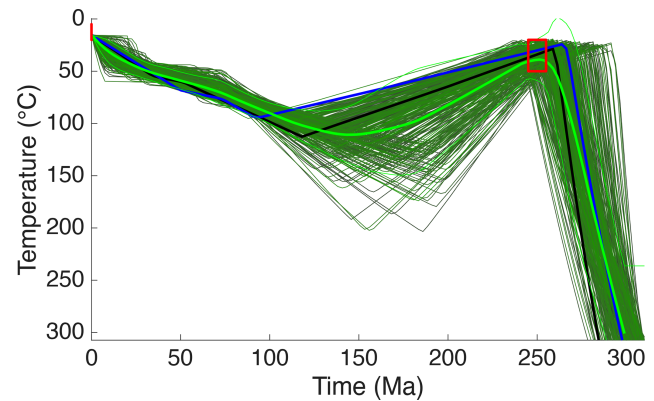
Figure 7. Modelled t – T -path of sample 22BGE055T using apatite fission track and in-situ (U-Th) / He data. Paths are color-ranked according to their fit from black to light green with the thick green line is the weighted mean cooling paths with 95 % CI (thin green lines). The t – T -path that fit best the data is shown in blue (highest summed GOF) and black (most input data fitted with \text{GOF} > 0.05 ). The red box is constraining the cooling paths to represent late Permian exhumation to near surface temperatures.
