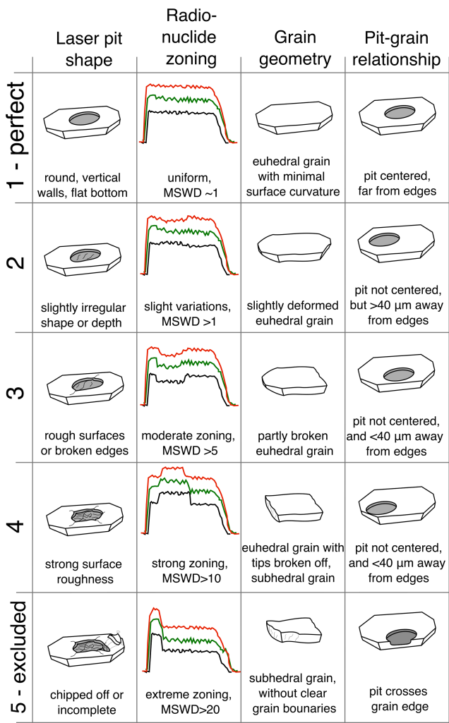
Figure 6. Decision matrix to rank/exclude in-situ (U-Th) / He measurements. The red, green and black lines in the second column (Radionuclide zoning) represent counts measured by LA-ICP-MS for trace elements such as radionuclides (U, Th, Sm).
