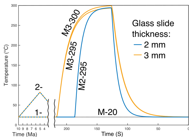
Figure 2. Time–temperature ( t – T ) path used to model the impact of our mounting protocol on apatite fission track annealing and He diffusion. Model scenarios include no pre-mounting heating (1–) and linear heating to 80 °C at 5 Ma (2–), followed by mounting t – T paths for glass thicknesses of 2 and 3 mm (M2, M3) and hot plate/press temperatures of 295 to 320 °C. For comparison an unrealistic mounting temperature of 20 °C is assumed (scenarios M-20).
