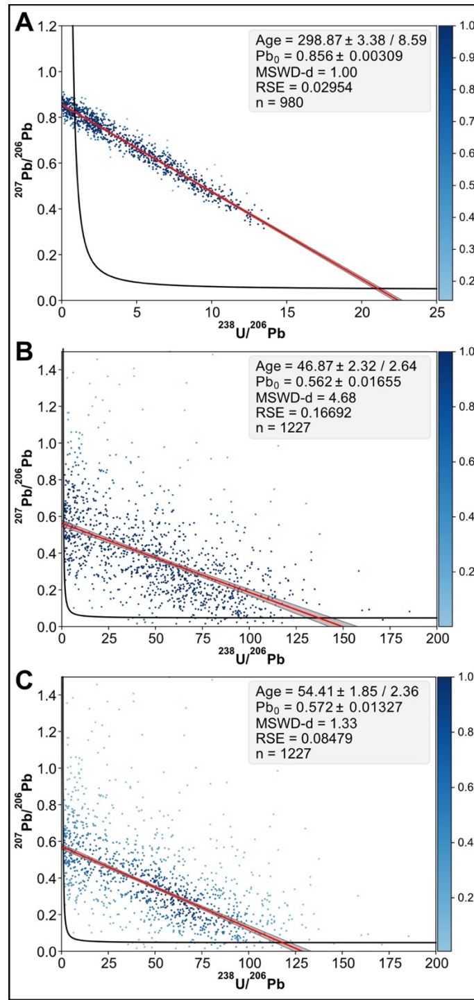
695 Figure 6: Results obtained for samples JS4 (A) and BM18 (B,C). A: TW concordia plot calculated by robust regression for sample JS4. B, C: TW concordia plots calculated by robust regression for sample BM18. In C, the robust regression is weighted, with pixel weights calculated from a 2D Kernel Density Estimate (see text for details).
