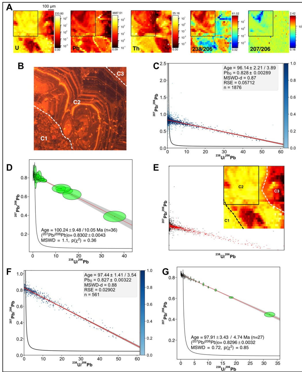
Figure 6: Results obtained for sample ETC2. A : Semi-quantitative element concentrations in ppm (U, Pb, Th) and ^{238}\text{U}/^{206}\text{Pb} , ^{207}\text{Pb}/^{206}\text{Pb} isotopic maps. Black frames correspond to the image subset selected by colocalization. B : TW concordia plot with ages and their uncertainty calculated by robust regression for the entire map. C : Cathodoluminescence image of an area close to that of the image map. Three distinct cements are distinguished (C1 to C3). C : B: TW concordia plot with ages and their uncertainty calculated by robust regression for the entire map. D : TW concordia plot calculated from discretization of the entire isotopic map ('pseudo-spots'). E : ^{207}\text{Pb}/^{206}\text{Pb} versus ^{238}\text{U}/^{206}\text{Pb} scatterplot obtained with the ScatterJn plugin from the isotopic maps. Red dots correspond to the pixels of the image subset (black frame in A and on the Uranium concentration map where the approximate location of distinct cement is given). F : TW concordia plot with ages and their uncertainty calculated by robust regression for the image subset. G : TW concordia plot obtained with the approach of Drost et al. (2018) for the entire isotopic map.
