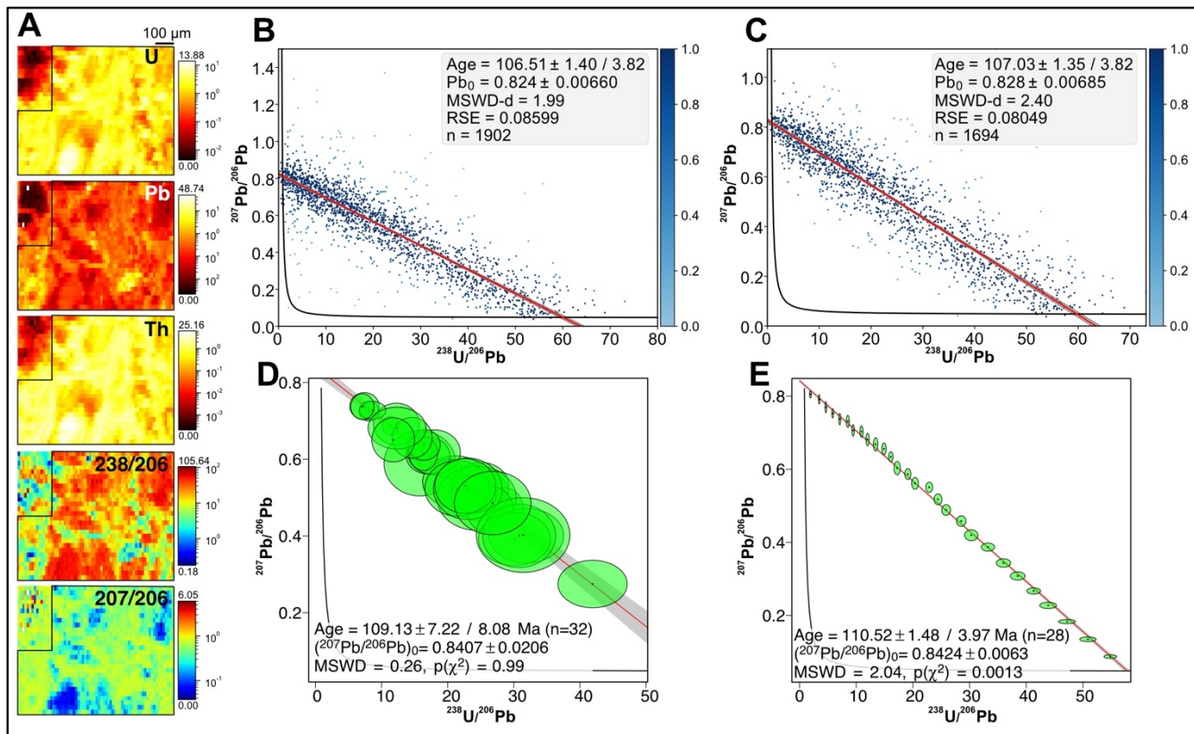
Figure 7: Results obtained for sample ARB. A: Semi-quantitative element concentrations in ppm (U, Pb, Th) and ^{238}\text{U}/^{206}\text{Pb} , ^{207}\text{Pb}/^{206}\text{Pb} isotopic maps. B: TW concordia plot with ages and their uncertainty calculated by robust regression. C: Same as B, except that TW concordia plot with pseudo-ellipses used for calculation of the d MSWD. Age and associated uncertainty obtained by York-type regression using IsoplotR are also indicated. The pixels outside the black frames on the isotopic maps (A) were not considered in age calculation, based on the colocalization study. D: TW concordia plot calculated from discretization of the entire isotopic map ('pseudo-spots'). G: TW concordia plot obtained with the approach of Drost et al. (2018) for the entire isotopic map.
