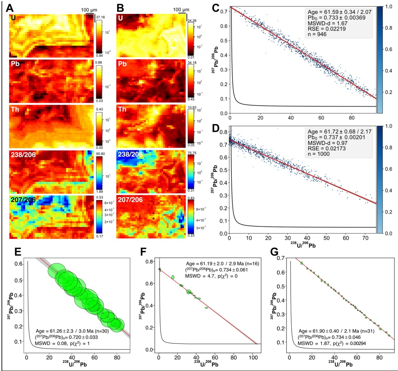
Figure 3: Results obtained for two isotopic maps of sample BH14 (A, C, E, G: first map; B, D, F: second map). A, B: Semi-quantitative element concentrations in ppm (U, Pb, Th) and ^{238}U/^{206}Pb , ^{207}Pb/^{206}Pb isotopic maps. C, D: TW concordia plots with ages and their uncertainty calculated by robust regression. E, F: TW concordia plots with age and its uncertainty calculated from discretization of the isotopic map ('pseudo-spots') ellipses used for calculation of the d-MSWD, with age and associated uncertainty (without systematic uncertainties) obtained by York-type regression using IsoplotR also indicated. G: TW concordia plot obtained from LA-ICP-MS spot analyses. G: TW concordia plot obtained with the approach of Drost et al. (2018). For E, F, G and similar plots in the next figures, Ages and associated uncertainties were obtained from York-type regression using IsoplotR (age uncertainties (1.96 \sigma level) are without (left) and with systematic uncertainty (right)).
