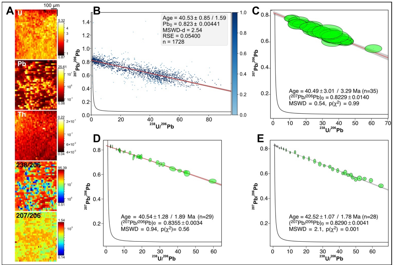
Figure 4: Results obtained for sample PXG20-1. A : Semi-quantitative element concentrations in ppm (U, Pb, Th) and ^{238}\text{U}/^{206}\text{Pb} , ^{207}\text{Pb}/^{206}\text{Pb} isotopic maps. B , C : TW and 86TW-plots with ages and their uncertainty calculated by robust regression. C : TW concordia plot calculated from discretization of the isotopic map ('pseudo-spots'). D : TW concordia plot with pseudo-ellipses used for calculation of the d-MSWD. Age and associated uncertainty obtained by York-type regression using IsoplotR are also indicated. E : TW concordia plot obtained from LA-ICP-MS spot analyses. Ages and associated uncertainties were obtained from York-type regression using IsoplotR. E : TW concordia plot obtained with the approach of Drost et al. (2018).
