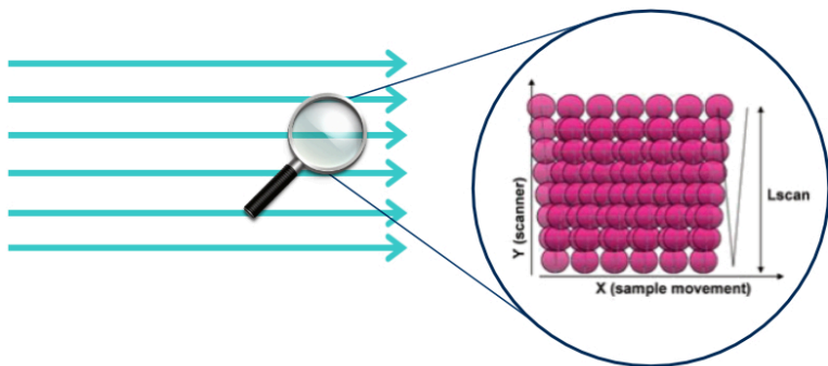
Figure 1: A: Principle of the construction of the ablation lines with the femtosecond laser used in the study. Lscan corresponds to the width of the line, here 50 \mu\text{m} or 25 \mu\text{m} . B: Example of ablation produced by the rasters used for producing an isotopic map (dimensions: 800 \mu\text{m} x 800 \mu\text{m} ).
