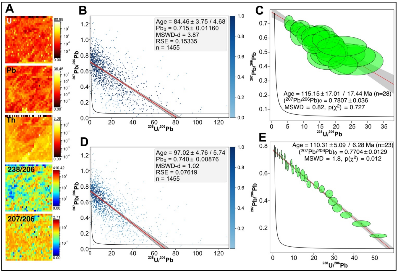
Figure 79: Results obtained for sample C6-265-D5. A: Semi-quantitative element concentrations in ppm (U, Pb, Th) and ^{238}\text{U}/^{206}\text{Pb} , ^{207}\text{Pb}/^{206}\text{Pb} isotopic maps. B: TW concordia plot with ages and their uncertainty calculated by robust regression. Pixels with ^{238}\text{U}/^{206}\text{Pb} and ^{207}\text{Pb}/^{206}\text{Pb} values above 130 and 1.3, respectively, are not shown ( n = 13 ). C: TW concordia plot calculated from discretization of the isotopic map ('pseudo-spots'). D: TW concordia plots calculated by weighted robust regression, with pixel weights calculated from a 2D Kernel Density Estimate. E: TW concordia plot obtained with the approach of Drost et al. (2018).
