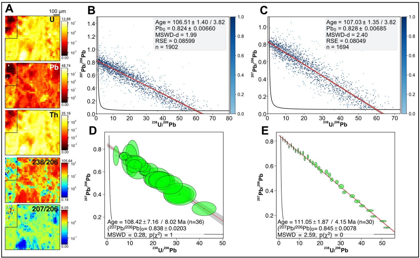
Figure 78: Results obtained for sample ARB. A: Semi-quantitative element concentrations in ppm (U, Pb, Th) and ^{238}\text{U}/^{206}\text{Pb} , ^{207}\text{Pb}/^{206}\text{Pb} isotopic maps. B: TW concordia plot with ages and their uncertainty calculated by robust regression. Pixels with ^{238}\text{U}/^{206}\text{Pb} and ^{207}\text{Pb}/^{206}\text{Pb} values above 80 and 1.4, respectively, are not shown ( n = 11 ). C: Same as B, except that the pixels outside the black frames on the isotopic maps (A) were not considered in age calculation, based on the colocalization study. D: TW concordia plot calculated from discretization of the entire isotopic map ('pseudo-spots'). G: TW concordia plot obtained with the approach of Drost et al. (2018) for the entire isotopic map.
