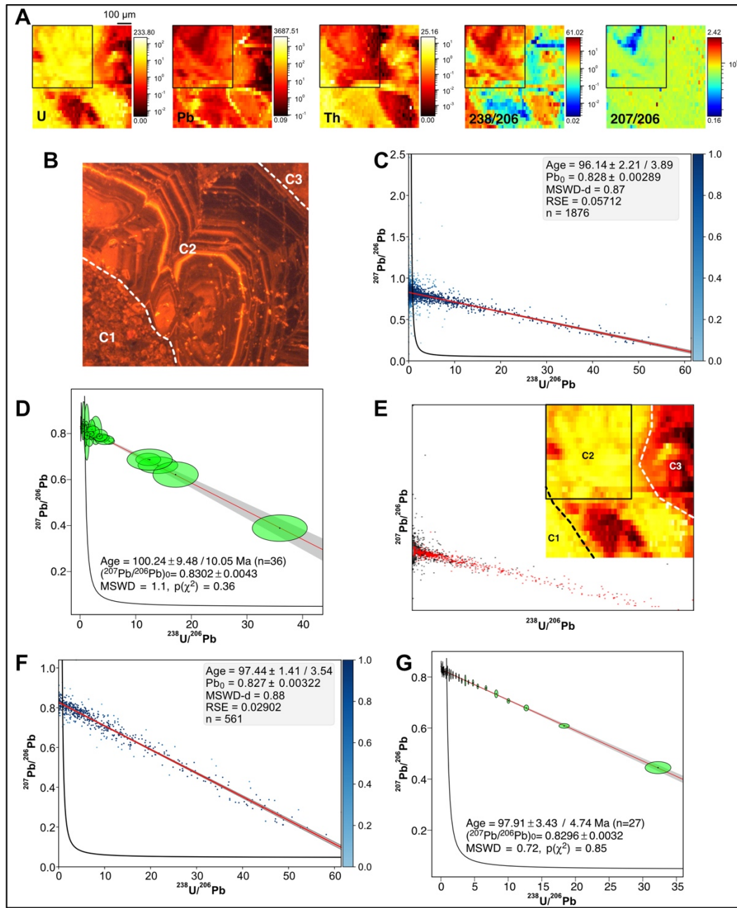
Figure 67: Results obtained for sample ETC2. A: Semi-quantitative element concentrations in ppm (U, Pb, Th) and ^{238}\text{U}/^{206}\text{Pb} , ^{207}\text{Pb}/^{206}\text{Pb} isotopic maps. Black frames correspond to the image subset selected by colocalization. B: Cathodoluminescence image of an area close to that of the image map. Three distinct cements are distinguished (C1 to C3). C: ^{207}\text{Pb}/^{206}\text{Pb} versus ^{238}\text{U}/^{206}\text{Pb} scatterplot obtained with the ScatterJn plugin from the isotopic maps. Red dots correspond to the pixels of the image subset (black frame in A and on the Uranium concentration map where the approximate location of distinct cement is given). D: TW concordia plot calculated from discretization of the entire isotopic map ("pseudo-spots"). E: ^{207}\text{Pb}/^{206}\text{Pb} versus ^{238}\text{U}/^{206}\text{Pb} scatterplot obtained with the ScatterJn plugin from the isotopic maps. Red dots correspond to the pixels of the image subset (black frame in A and on the Uranium concentration map where the approximate location of distinct cement is given). F: TW concordia plot with ages and their uncertainty calculated by robust regression for the image subset. G: TW concordia plot obtained with the approach of Drost et al. (2018) for the entire isotopic map.
