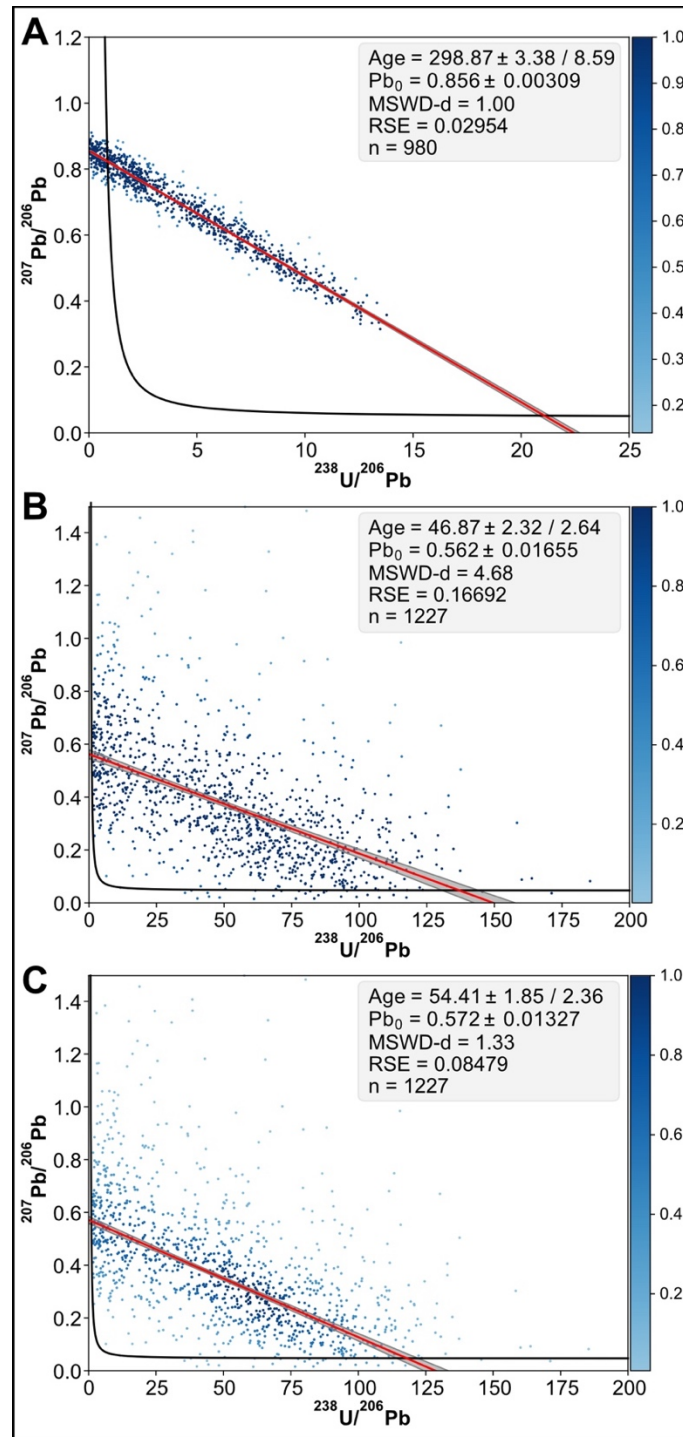
655 Figure 6: Results obtained for samples JS4 (A) and BM18 (B,C). A: TW concordia plot calculated by robust regression for sample JS4. B, C: TW concordia plots calculated by robust regression for sample BM18. In C, the robust regression is weighted, with pixel weights calculated from a 2D Kernel Density Estimate (see text for details).
