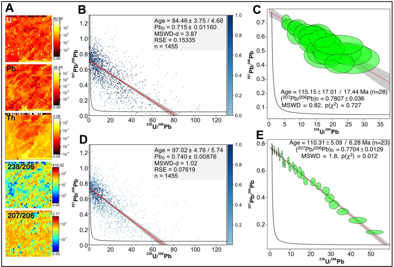
Figure 7: Results obtained for sample C6-265-D5. A: Semi-quantitative element concentrations in ppm (U, Pb, Th) and ^{238}\text{U}/^{206}\text{Pb} , ^{207}\text{Pb}/^{206}\text{Pb} isotopic maps. B: TW concordia plot with ages and their uncertainty calculated by robust regression. C: TW concordia plot calculated from discretization of the isotopic map ('pseudo-spots'). D: TW concordia plots calculated by weighted robust regression, with pixel weights calculated from a 2D Kernel Density Estimate. E: TW concordia plot obtained with the approach of Drost et al. (2018).
