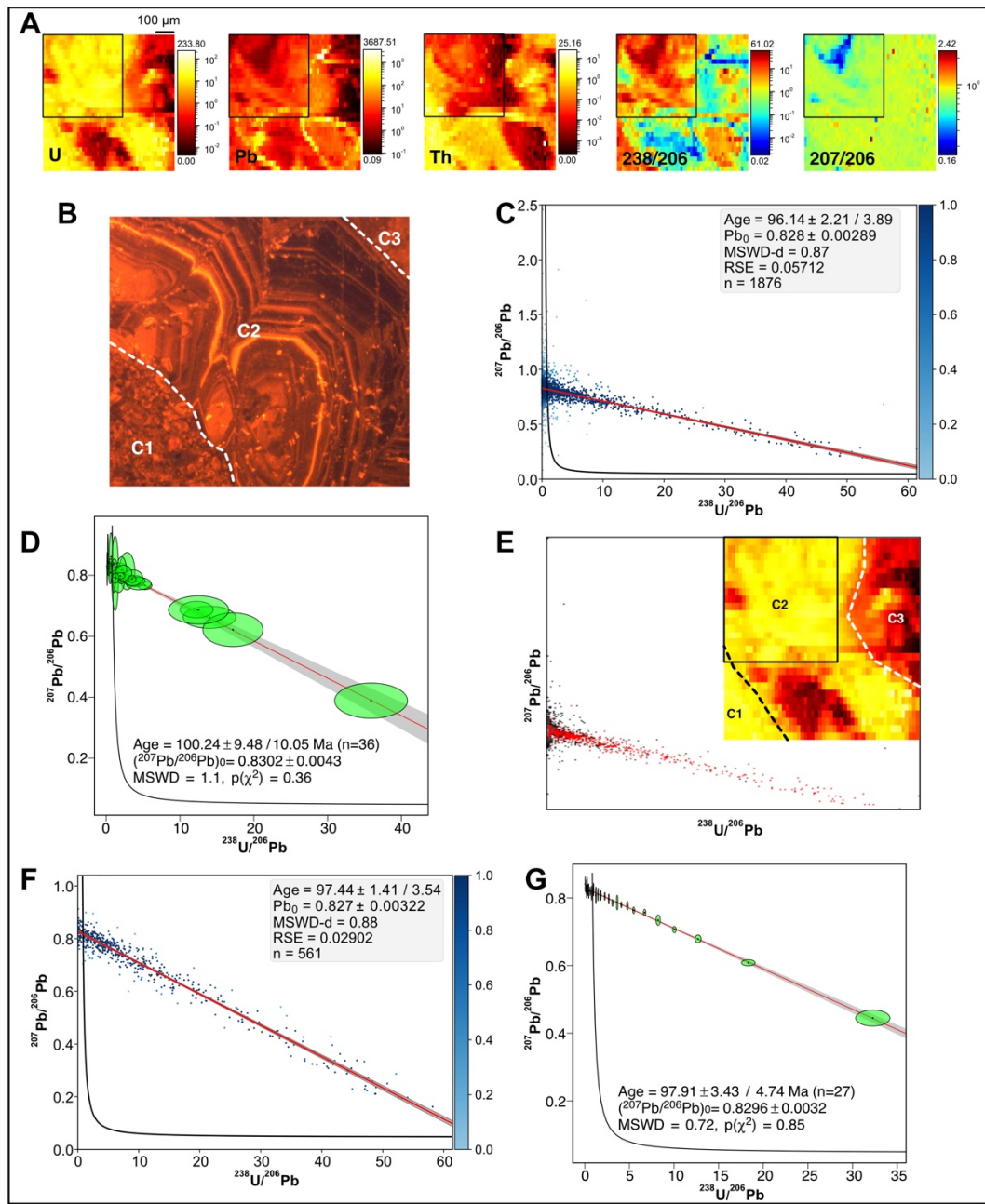
Figure 6: Results obtained for sample ETC2. A: Semi-quantitative element concentrations in ppm (U, Pb, Th) and ^{238}\text{U}/^{206}\text{Pb} , ^{207}\text{Pb}/^{206}\text{Pb} isotopic maps. Black frames correspond to the image subset selected by colocalization. B: Cathodoluminescence image of an area close to that of the image map. Three distinct cements are distinguished (C1 to C3). C: B: TW concordia plot with ages and their uncertainty calculated by robust regression for the entire map. D: TW concordia plot calculated from discretization of the entire isotopic map ("pseudo-spots"). E: ^{207}\text{Pb}/^{206}\text{Pb} versus ^{238}\text{U}/^{206}\text{Pb} scatterplot obtained with the ScatterJn plugin from the isotopic maps. Red dots correspond to the pixels of the image subset (black frame in A and on the Uranium concentration map where the approximate location of distinct cement is given). F: TW concordia plot with ages and their uncertainty calculated by robust regression for the image subset. G: TW concordia plot obtained with the approach of Drost et al. (2018) for the entire isotopic map.
