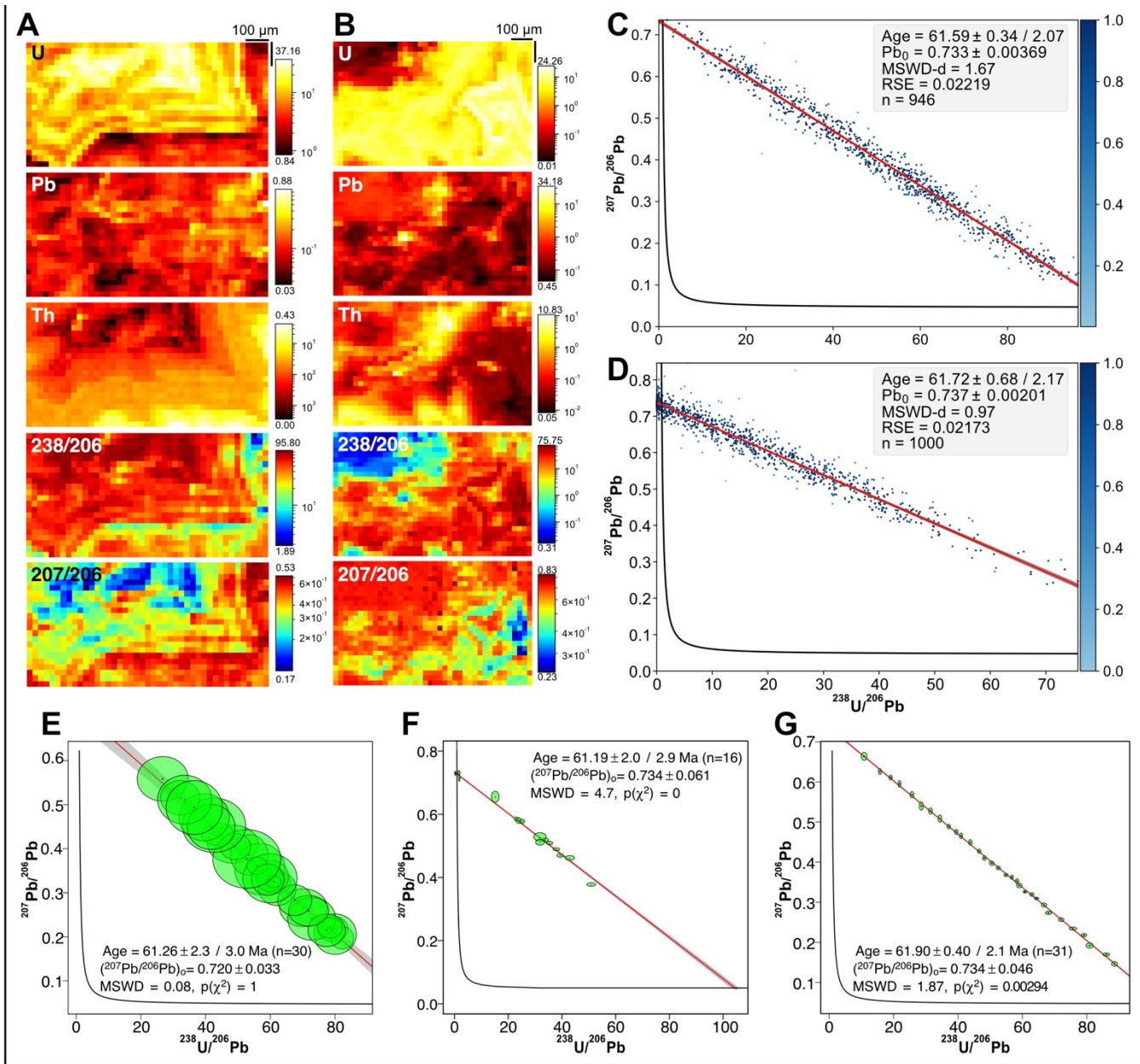
Figure 3: Results obtained for two isotopic maps of sample BH14 (A, C, E, G: first map; B, D: second map). A, B: Semi-quantitative element concentrations in ppm (U, Pb, Th) and ^{238}U/^{206}Pb , ^{207}Pb/^{206}Pb isotopic maps. C, D: TW concordia plots with ages and their uncertainty calculated by robust regression. E: TW concordia plot with age and its uncertainty calculated from discretization of the isotopic map ('pseudo-spots'). F: TW concordia plot obtained from LA-ICP-MS spot analyses. G: TW concordia plot obtained with the approach of Drost et al. (2018). For E, F, G and similar plots in the next figures, ages and associated uncertainties were obtained from York-type regression using IsoplotR (age uncertainties ( 1.96\sigma level) are without (left) and with systematic uncertainty (right)).
