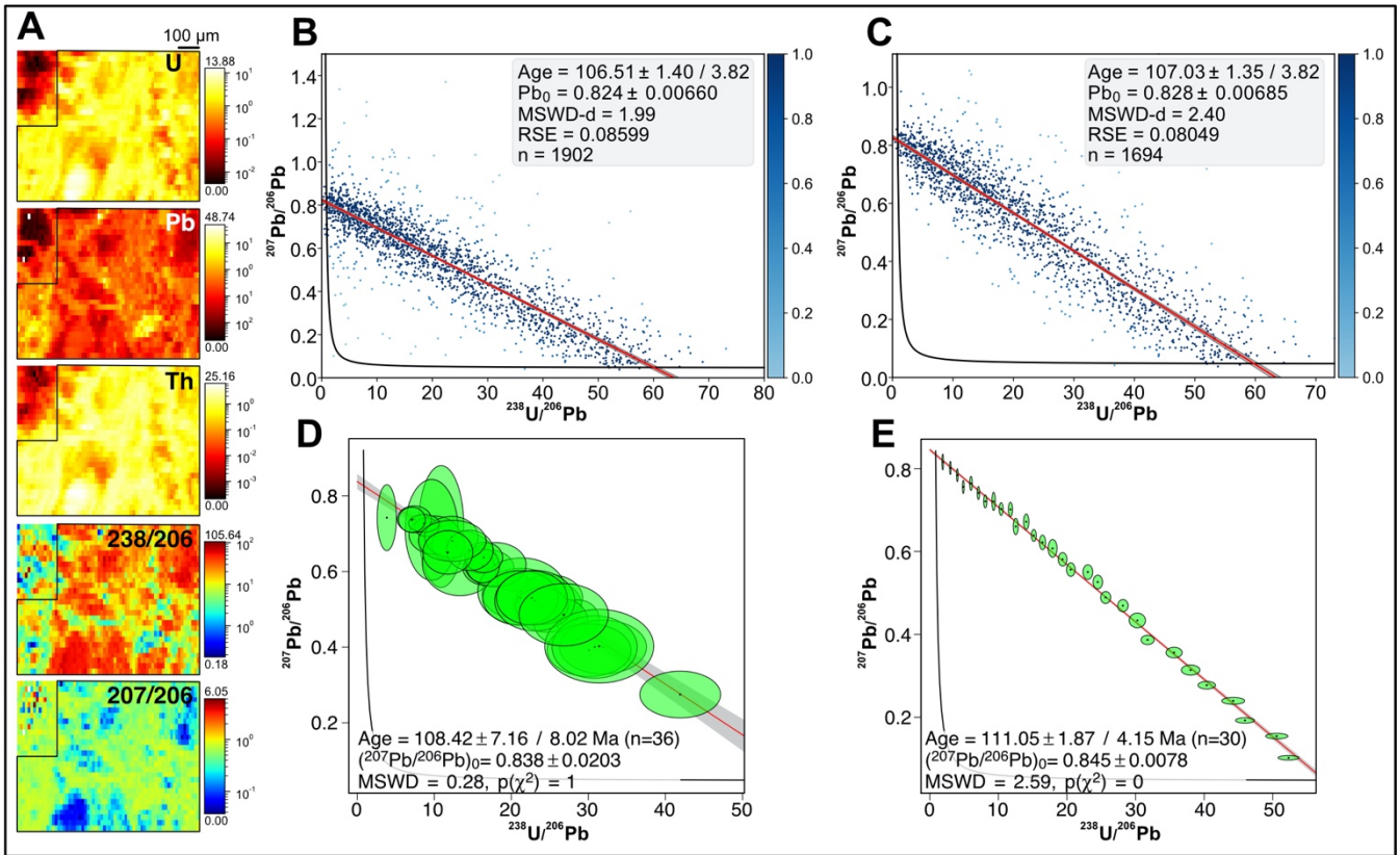
675 Figure 8: Results obtained for sample ARB. A: Semi-quantitative element concentrations in ppm (U, Pb, Th) and ^{238}\text{U}/^{206}\text{Pb} , ^{207}\text{Pb}/^{206}\text{Pb} isotopic maps. B: TW concordia plot with ages and their uncertainty calculated by robust regression. Pixels with ^{238}\text{U}/^{206}\text{Pb} and ^{207}\text{Pb}/^{206}\text{Pb} values above 80 and 1.4, respectively, are not shown ( n = 11 ). C: Same as B, except that the pixels outside the black frames on the isotopic maps (A) were not considered in age calculation, based on the colocalization study. D: TW concordia plot calculated from discretization of the entire isotopic map ('pseudo-spots'). G: TW concordia plot obtained with the approach of Drost et al. (2018) for the entire isotopic map. 680
