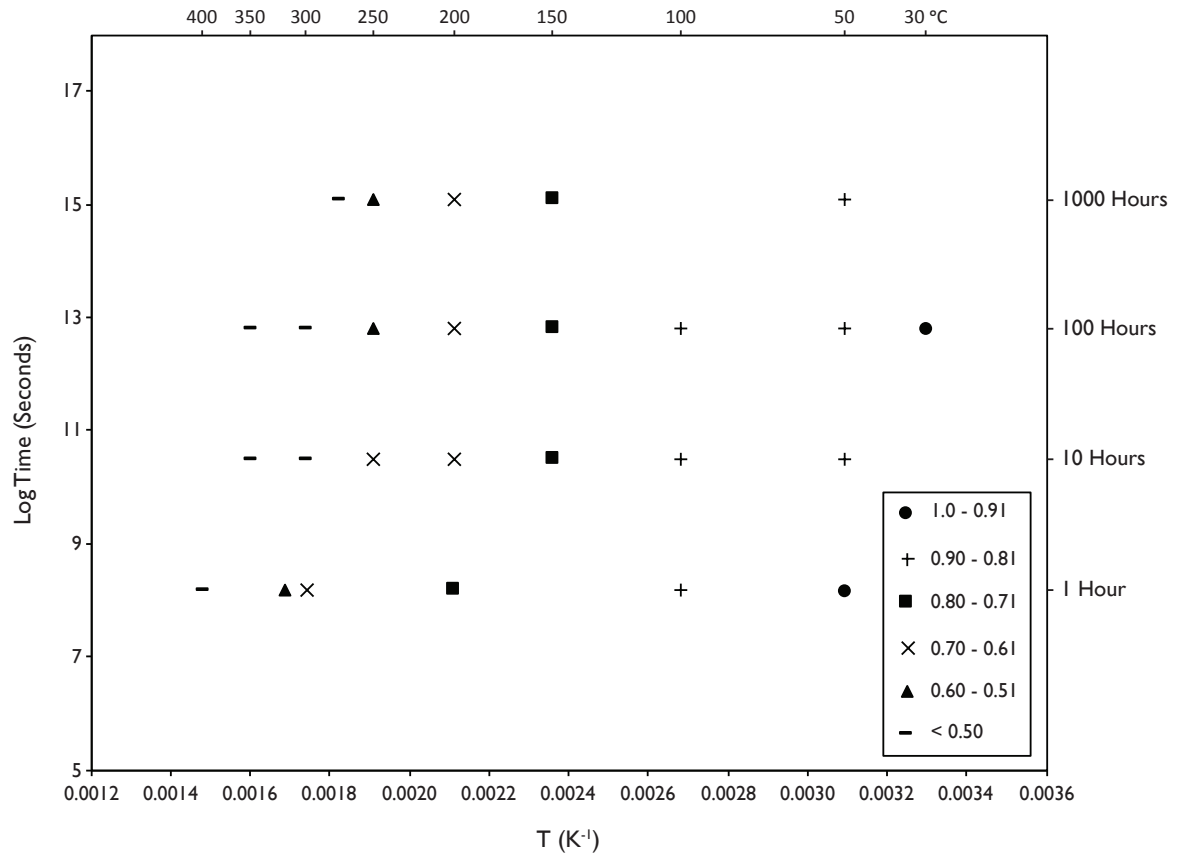
Figure 7. Arrhenius plot of experimental data using calculated equivalent confined fission track lengths in Harcourt Granodiorite monazite. Each point represents two annealing experiments that have been averaged across both orientations ( \parallel and \perp surfaces, as in Figure 4). Different degrees of track length reduction ( r ) are shown by different symbols. Inverse absolute temperature in Kelvins shown on the x-axis and corresponding temperatures in ^{\circ}\text{C} along the top.
