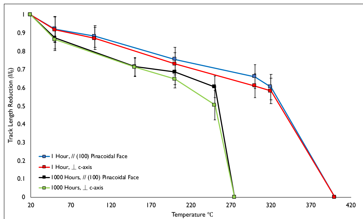
Figure 5. Normalized track length reduction ( l/l_0 ) against temperature for calculated equivalent confined fission tracks for 1 and 1000 hour experiments for both surface orientations ( // and \perp surfaces, as in Figure 4). The normalized track length ( l/l_0 ) values are calculated from the average length of the control samples ( 10.60 \mu\text{m} ). Error bars refers to 1\sigma errors.
