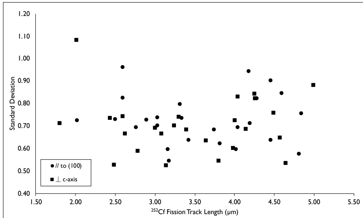
Figure 6. Standard deviation of 252 Cf fission-track length distributions plotted against their average track lengths for both parallel and perpendicular surfaces across all experiments.
