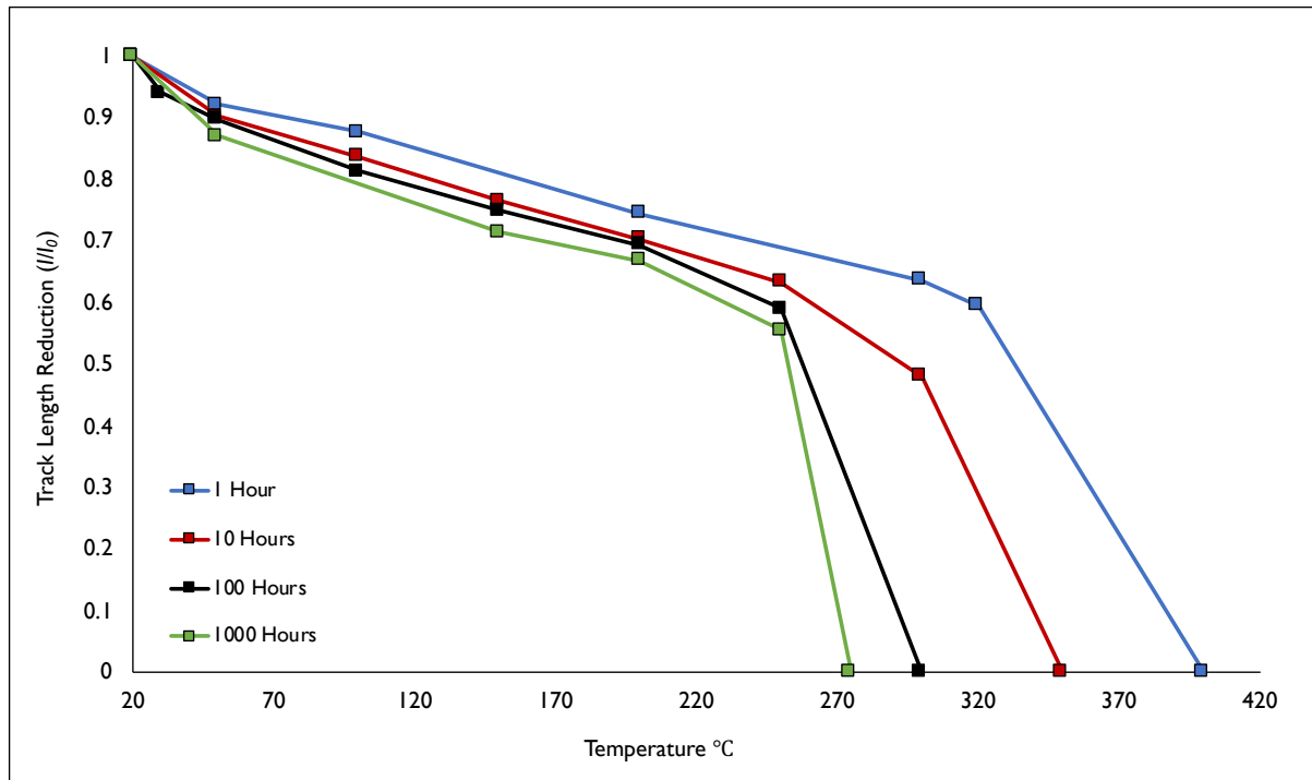
Figure 4. Normalized track length reduction ( l/l_0 ) against temperature for calculated equivalent confined fission tracks in Harcourt Granodiorite monazite. The track length reduction values are averaged across both sets of surfaces ( // to (100) and \perp to the c-axis) with the normalized track length ( l/l_0 ) values being calculated from the average length of the unannealed control samples ( 10.60 \mu\text{m} ).
