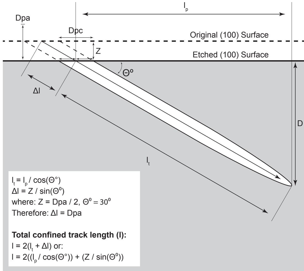
Figure 3. Illustration of the measurements and calculations required to correct semi-track lengths for surface etching on a (100) face (ie parallel to b and c). Bulk etching removes the original surface by approximately half the width of the etch pit diameter parallel to the a-axis ( Dpa ) measured on the \sim(001) face (modified from Ure 2010).
