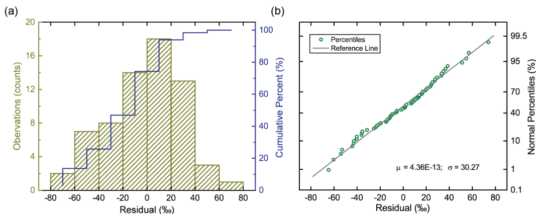
Figure 2: Histogram (left) and normal percentiles plot (right) of the residual. The reference line in the right plot refers to the line of standard normal distribution.
