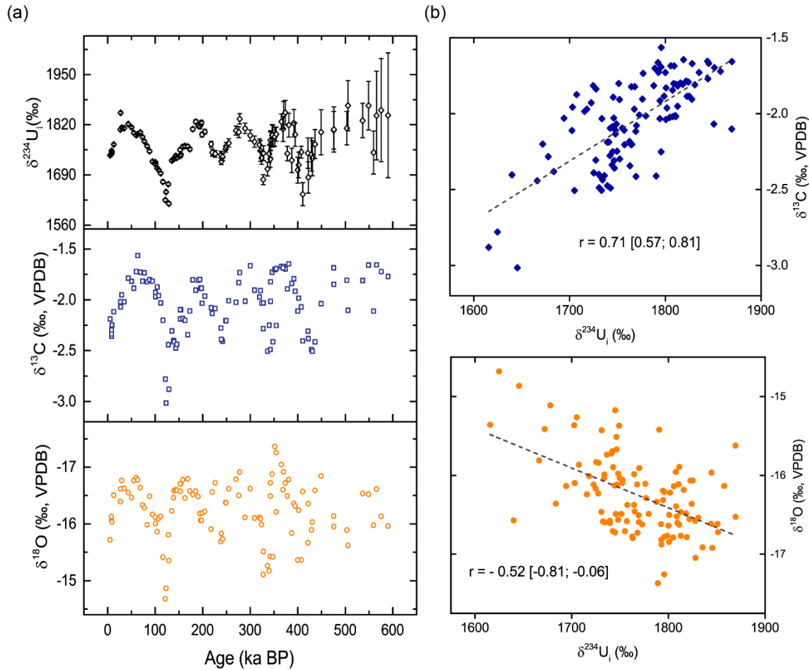
150 Figure 1: (a) Plots of DH2 ^{230}\text{Th} -derived \delta^{234}\text{U}_i , \delta^{13}\text{C} , and \delta^{18}\text{O} over the last 590 ka BP; (b) scatter plots between DH2 ^{230}\text{Th} -derived \delta^{234}\text{U}_i and \delta^{13}\text{C} , and ^{230}\text{Th} -derived \delta^{234}\text{U}_i and \delta^{18}\text{O} respectively. Correlation coefficients (r) with 95% calibrated confidence intervals and fitting curve (dashed lines) are shown.
