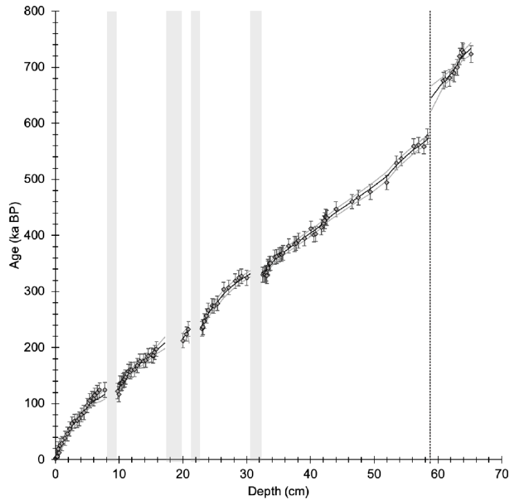
250 Figure 5: ^{234}\text{U} ages (diamonds) and associated 2\sigma uncertainties along the length of the core penetrating the calcite crust. OxCal age model (black line) and 95 % confidence limits (grey lines) were derived from ^{234}\text{U} ages. Location of folia (grey bars) and a growth hiatus (black dashed line) are indicated.
