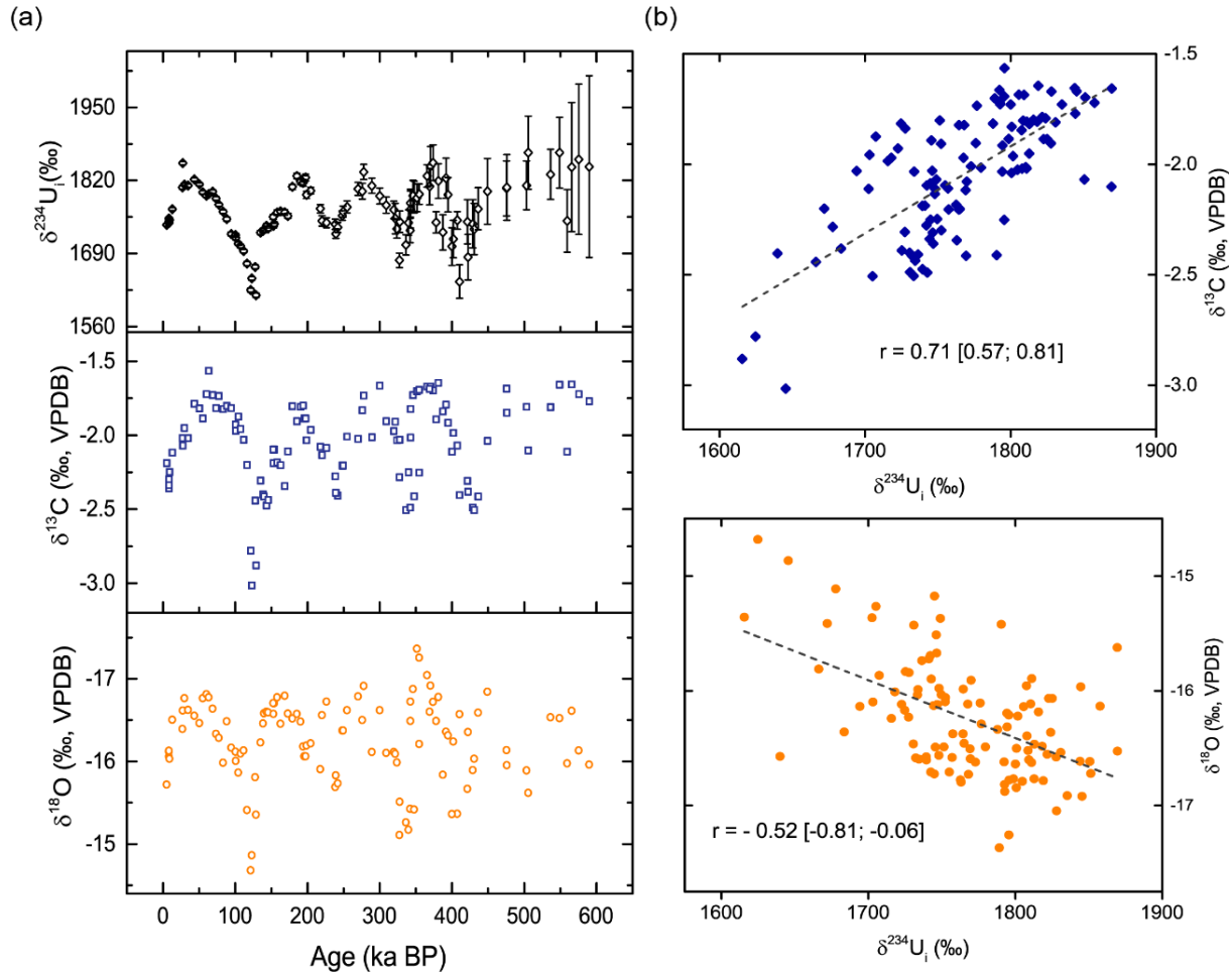
Figure 1: (a) Plots of DH2 ^{230}\text{Th} -derived \delta^{234}\text{U}_i , \delta^{13}\text{C} , and \delta^{18}\text{O} over the last 590 ka BP; (b) scatter plots between DH2 ^{230}\text{Th} -derived \delta^{234}\text{U}_i and \delta^{13}\text{C} , and ^{230}\text{Th} -derived \delta^{234}\text{U}_i and \delta^{18}\text{O} respectively. Correlation coefficients ( r ) with 95% calibrated confidence intervals and fitting curve (dashed lines) are shown.
