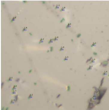
Figure 3: example of semi-automatic D_{00r} measurement result obtained on a part of an image taken on 1000x magnification. The green ellipses are the remainders from a segmentation process. The values written next to the ellipses stand for length in \mu\text{m} (black), elongation factor (red) and angle (blue). Some green ellipses show no values because they have been excluded by the elongation filter, direction filter, minimum size filter or maximum size filter.
