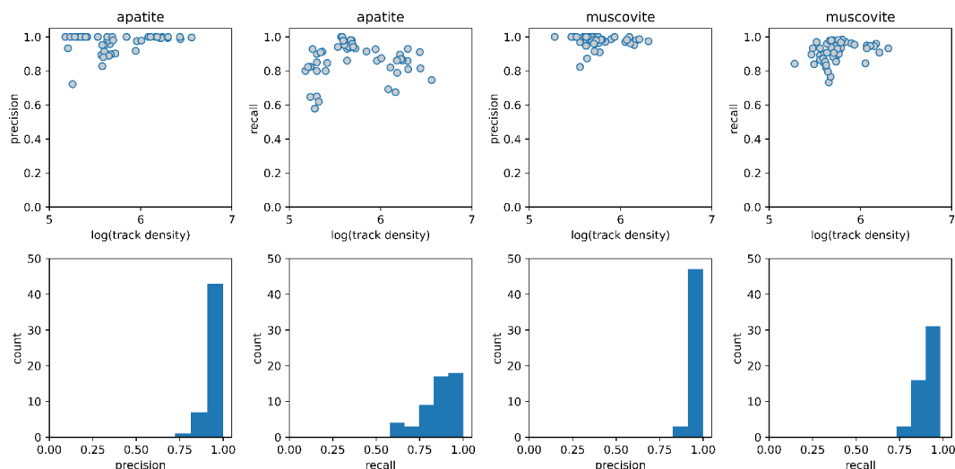
Figure 4: Performance metrics of the deep neural networks obtained on a dataset containing 50 “test images”. The precision (true positives/(true positives + false positives)) and recall (true positives/(true positives + false negatives)) of the automatic fission track recognition deep neural network are shown for apatite and muscovite mica (external detector). The 10-based log of areal track density (tracks/ \text{cm}^2 ) is shown on the horizontal axis of the upper scatter plots. The frequency-histograms below show the distribution of the performance metrics.
