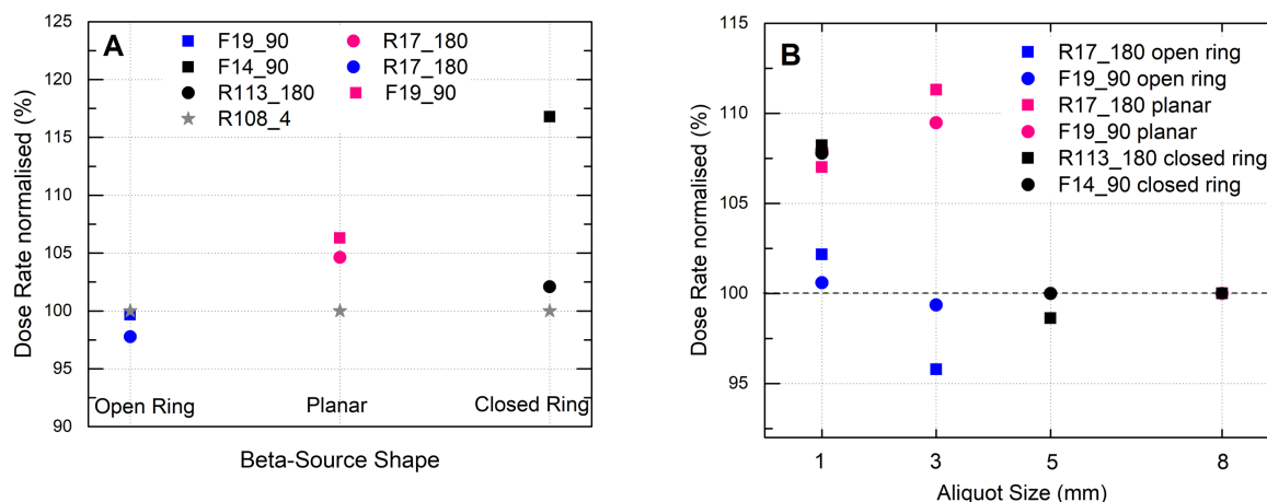
Fig. 3. Experimentally determined normalised beta-dose rates. A - dose rate normalised to the respective figure value (sample R108_4) versus beta-source shape; Aliquot size is 7.95 mm (R17_180; F19_90) or 5 mm (F14_90). B - dose rate normalised to 7.95 mm or 5 mm aliquot size plotted versus aliquot size. For the sake of clarity error bars are not plotted. For data and uncertainty see Table 3.
