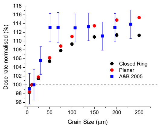
210 Fig. 5. Result from GEANT4 simulation compared to published experimental data. The dose rate is plotted as a function of grain size for the planar source and the closed-ring source and for experimental data (A&B 2005; Armitage and Bailey, 2005). Simulated data are normalised to the 10 \mu\text{m} grain size, aliquot size is
