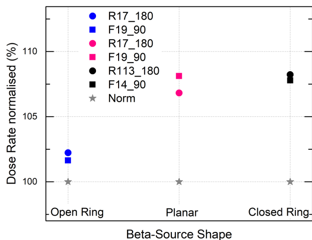
205 Fig. 4. Beta-dose rates of 1 mm aliquots normalised to the 7.95 or 5 mm aliquot size of the respective sample versus beta-source shape. For the sake of clarity error bars are not plotted. For data and uncertainty see Table 3.
