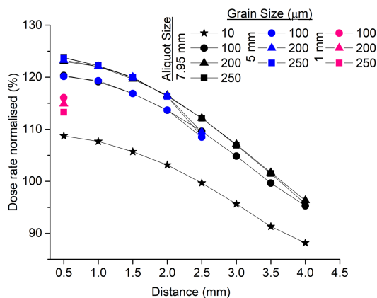
250 Fig. 8. Result from GEANT4 simulation: dose rate versus distance from centre of the stainless-steel cup for the closed-ring beta source. Data are for large (7.95 mm), medium (5 mm) and small (1 mm) aliquot sizes and for 10, 100, 200, 250 \mu\text{m} grain sizes. Dose rate is normalised to 10 \mu\text{m} grain size the average value of which is at 100%.
