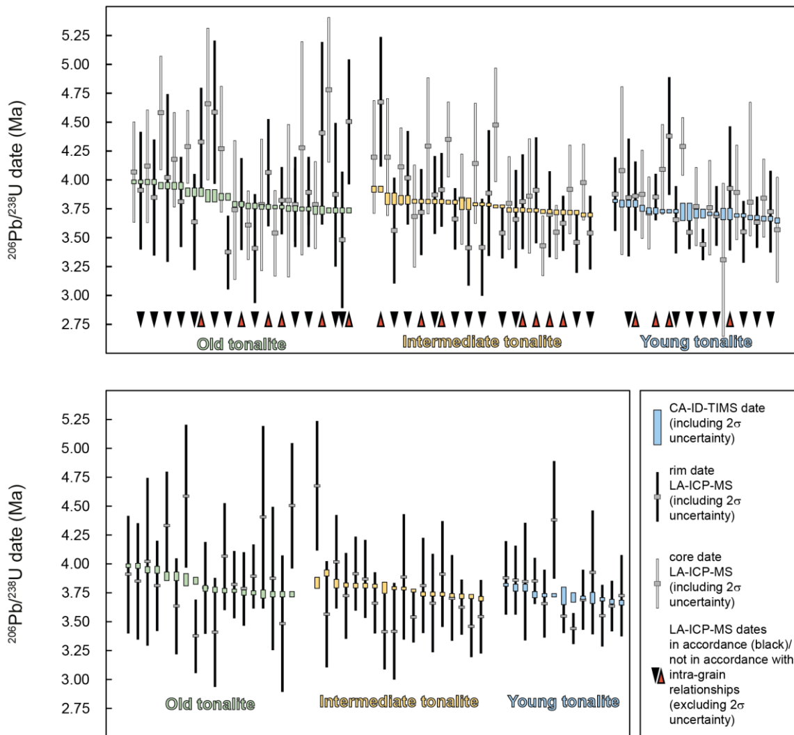
Figure 10: Comparison of in-situ LA-ICP-MS dates and CA-ID-TIMS dates on the same zircons. In upper panel each CA-ID-TIMS date is aligned with the rim (filled) and core (empty) LA-ICP-MS date of the same zircon. Coloured bars indicate individual CA-ID-TIMS analysis including analytical uncertainty ( 2\sigma ). Downward pointing black arrow indicates that core analyses are older than rim analyses of the respective zircon, whereas red upward pointing arrow indicates the opposite. Note that CA-ID-TIMS dates can be plotted several times, with core and rim analyses of the same zircon. Lower panel compares CA-ID-TIMS date with respective rim analysis.
