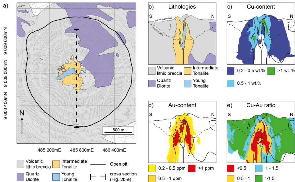
130 Figure 2: Geological map (a) and north to south cross-sections with lithological information and grade contours (b-e) of the open pit at Batu Hijau. The Intermediate and Young tonalite intruded into a Volcanic lithic breccia and the equigranular quartz diorite (a, b). Note that the extent of the Old tonalite is not displayed but is included in the Intermediate tonalite. Dashed line in a) is the N-S section displayed in b)-e). Thin grey lines in a) indicate mine-benches. Cu- and Au-grades (c + d) are enveloped around the tonalites and a deep, central barren core. High-grade Cu- and Au-mineralisation is cut by the Young tonalite. The ratios of Cu to Au (e) illustrate strong Au-enrichment proximal to the Intermediate tonalite and Cu-dominated distal mineralization. Map, section and grades are based on company information from May 2016. 135
