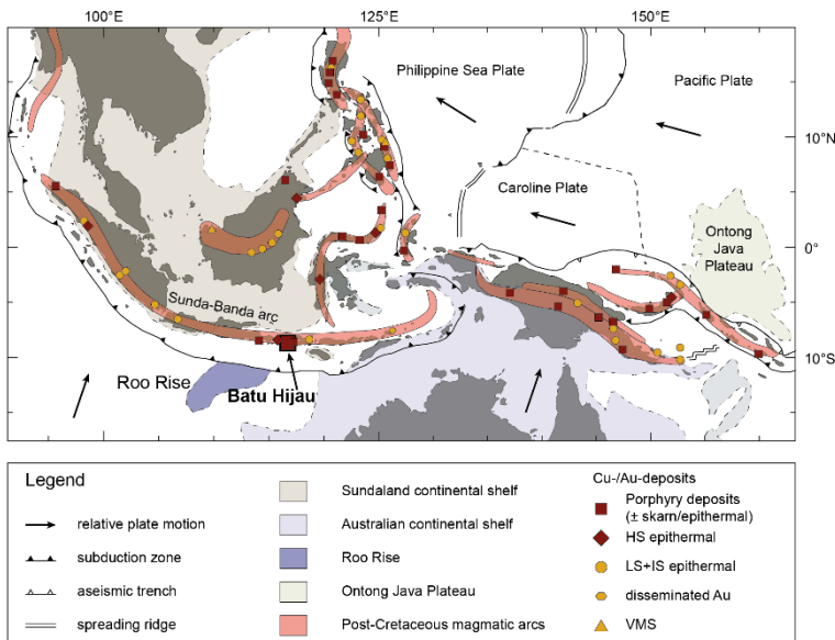
115 Figure 1: Tectonic map of southeast Asia and the southwest Pacific. The Batu Hijau porphyry Cu-Au deposit (enlarged red square) is located on Sumbawa on the subduction related, magmatic Sunda-Banda arc within a small corridor between 110°E and 120°E that hosts several porphyry deposits. Arrows display plate motion relative to the Eurasian plate (Sundaland shield) but do not indicate velocity. Abbreviations: HS = high sulphidation, IS – intermediate sulphidation, LS – intermediate sulphidation, VMS – volcanic hosted massive sulphide deposit. Most deposit locations are from Garwin (2005).
