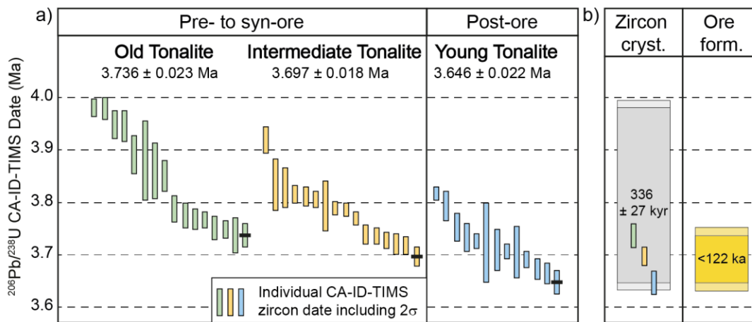
335 Figure 5: High-precision U-Pb CA-ID-TIMS zircon dates from the three tonalite porphyries and comparison with weighted mean averages by in-situ U-Pb geochronology. Vertical bars are individual analyses including analytical uncertainty ( 2\sigma ). The youngest crystallization age is used as the best approximation for porphyry emplacement. The extended range in zircon crystallization ages in each sample indicates protracted crystallization. Yellow box indicates 340 maximum duration of ore formation as constrained by the emplacement age of the Old tonalite and the Young tonalite. Grey box illustrates the duration of zircon crystallization recorded by CA-ID-TIMS geochronology. Vertical bars in the grey box are emplacement ages of the tonalites, demonstrating >200 ka of zircon crystallization before emplacement of the first porphyry intrusion and start of Cu-Au mineralisation.
