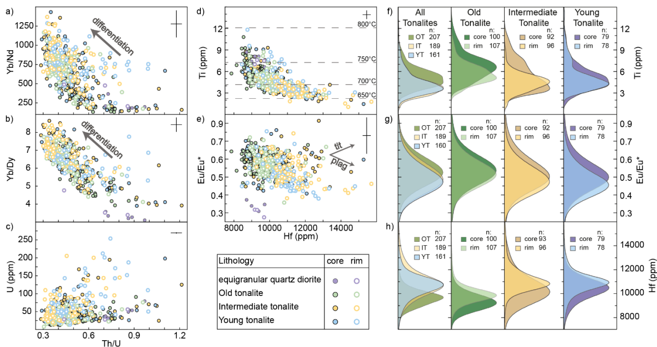
275 Figure 4: Covariation diagrams (a-e) and probability density plots (f-h) of in-situ geochemical data obtained by LA-ICP-MS. a) - c) are plotted against Th/U as an indicator for fractionation, whereas d) + e) are plotted against Hf as the fractionation proxy. Arrows labelled ‘fractional crystallisation’ indicate the approximate predicted direction zircon geochemistry would migrate given fractional crystallization of zircon ± apatite ± titanite ± amphibole. Arrows labelled ‘plag’ and ‘tit’ points into the predicted direction of zircon geochemistry evolution during co-crystallisation with plagioclase or titanite. Zircons from the three tonalite porphyries are considered to have crystallised from the same magma reservoir, whereas zircons from the equigranular quartz diorite (purple) are unrelated (see text for discussion). Temperature lines in d) are calculated with an assumed a\text{SiO}_2 = 1 and a\text{TiO}_2=0.7 based on Ferry and Watson (2007: see text for discussion). Cross in top right corners illustrates average analytical 2\sigma uncertainties. Probability density plots (after Vermeesch et al., 2013) illustrate differences between different samples and core and rim analyses within each sample. Axes of probability density plots in f) + g) are aligned with axes of d) + e). 280 285
