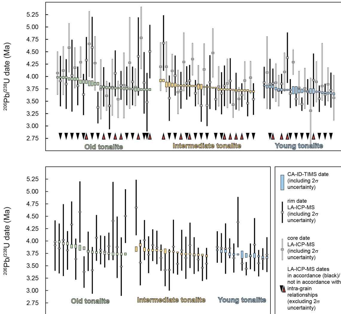
615 Figure 10: Comparison of in-situ LA-ICP-MS dates and CA-ID-TIMS dates on the same zircons. In upper panel each CA-ID-TIMS date is aligned with the rim (filled) and core (empty) LA-ICP-MS date of the same zircon. Coloured bars indicate individual CA-ID-TIMS analysis including analytical uncertainty ( 2\sigma ). Downward pointing black arrow indicates that core analyses are older than rim analyses of the respective zircon, whereas red upward pointing arrow indicates the opposite. Note that CA-ID-TIMS dates can be plotted several times, with core and rim analyses of the same zircon. Lower panel compares CA-ID-TIMS date with respective rim analysis.
