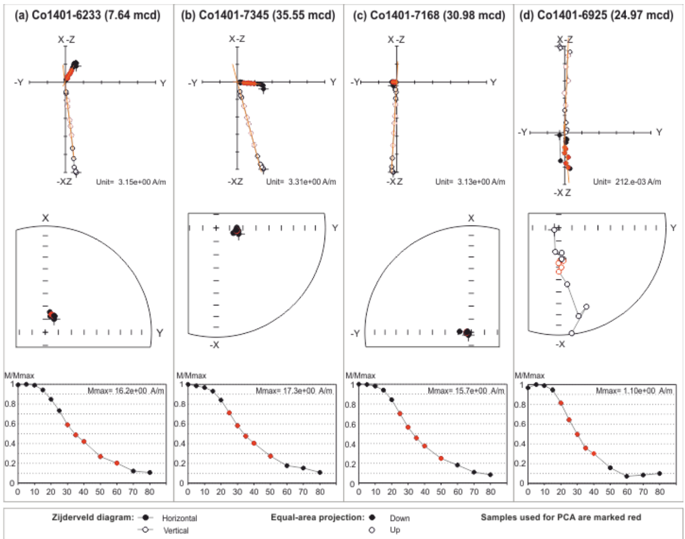
Fig. 4: AF demagnetization characteristics of selected samples. Zijdeveld diagrams, equal area projections and normalized NRM intensity are shown in the first, second, and third row, respectively. Points used to define the ChRM are marked in red.
