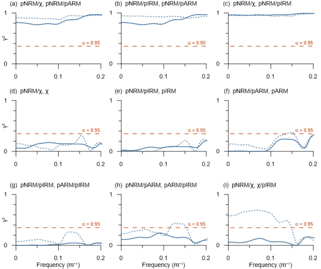
Fig. 5: Squared coherence \gamma^2 between RPI proxies and rock magnetic parameters for the whole depth range (dashed blue lines), for >6.7 mcd (solid blue lines), compared to the 95% confidence level threshold (dashed red lines). (a-c) Squared coherence between RPI proxies. (d-f) Squared coherence between RPI proxies and the corresponding NRM normalizer. (g-i) Squared coherence between RPI proxies and magnetic grain size indicators.
