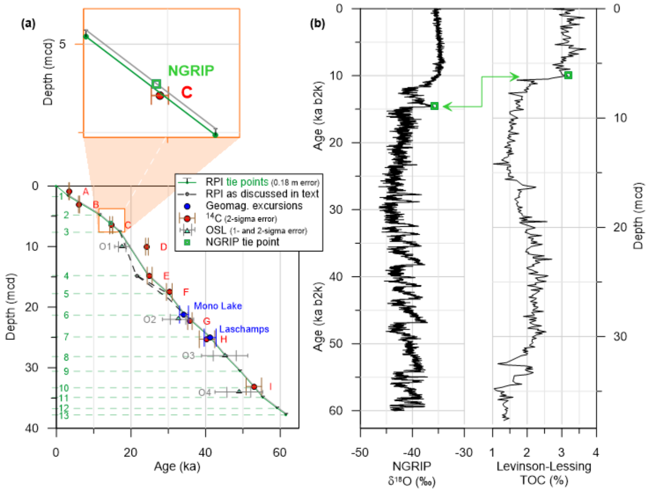
Fig. 8: (a) Age-depth model of the core composite Co1401. Ages of the geomagnetic excursions shown after Laj et al. (2014). The grey line represents the age-depth relationship resulting of a constant lock-in depth of 18 cm. The age of the NGRIP tie point results from the comparison of \delta^{18}\text{O} vs. age and TOC of Co1401 vs. depth (b). Its age is recalculated to BP ages.
