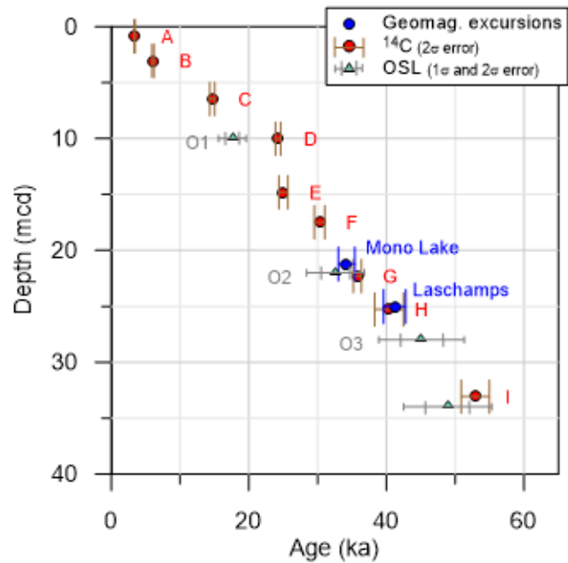
Fig. 2: OSL and AMS 14 C dating results of core composite Co1401, and locations of Laschamps and Mono Lake excursions. Ages and age uncertainties of the geomagnetic excursions are taken from Laj et al. (2014).
