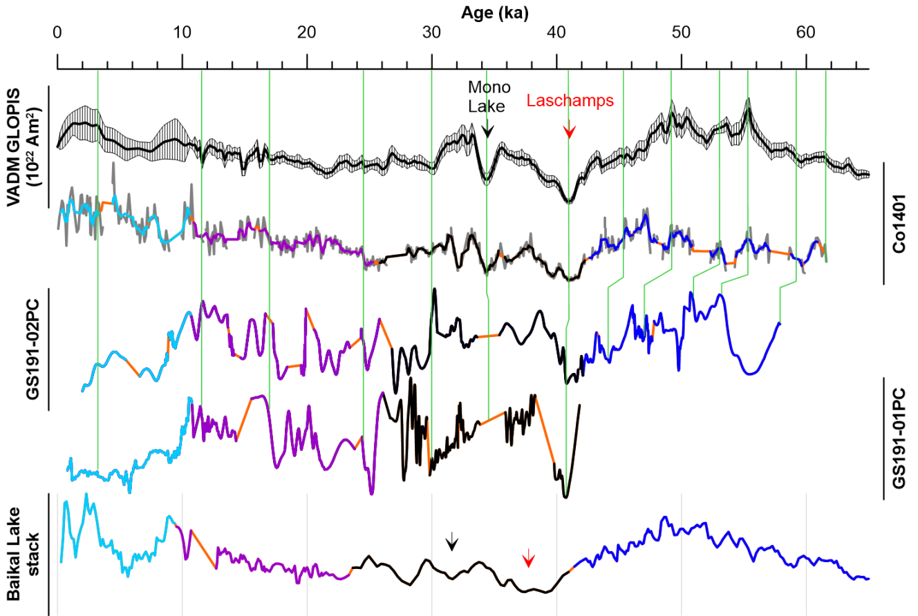
Fig. 9: Comparison of the smoothed RPI(IRM) of Co1401 (non-smoothed data in grey colours in the background) with RPI records from Lake Baikal (Baikal Lake stack) and the Barents Sea (GS191-01PC and GS191-02PC) and the VADM of GLOPIS-75-GICC05. All records are normalized to the respective maxima. For discussion, the RPI records are divided into four parts by colour code (light blue, purple, black, and royal blue). Gaps in the individual records are marked in orange. Please note the different ages assigned to the RPI characteristics of the different datasets, leading to a shift of the patterns against each other (c.f., section 3.4). Tie lines are shown as in Fig. 6. For the Baikal Lake stack, only the main grid lines are provided, as correlation is not readily possible. The locations of geomagnetic excursions are indicated by tie lines and arrows.
