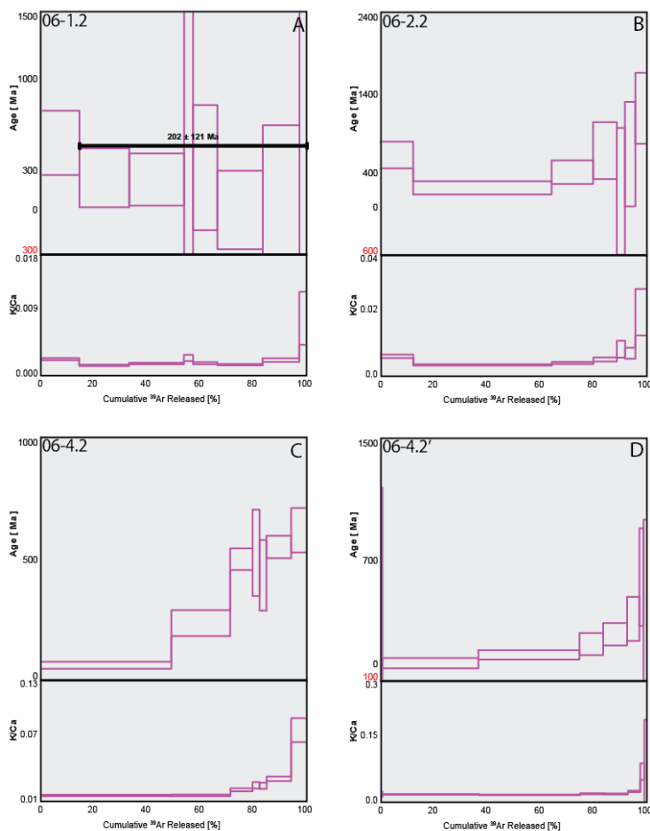
225 Fig. 6. Combined age spectra and K/Ca plots for samples 06-1.2 (A), 06-2.2 (B), 06-4.2 (C), 06-4.2' (D). The thickness of individual spectra blocks is indicative of measurement uncertainty.
