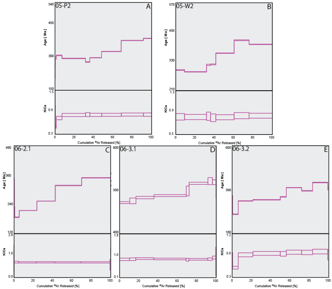
Fig. 5. Combined age spectra and K/Ca plots for samples 05-P2 (A), 05-W2 (B), 06-2.1 (C), 06-3.1 (D), 06-3.2 (E). The thickness of individual spectra blocks is indicative of measurement uncertainty.
