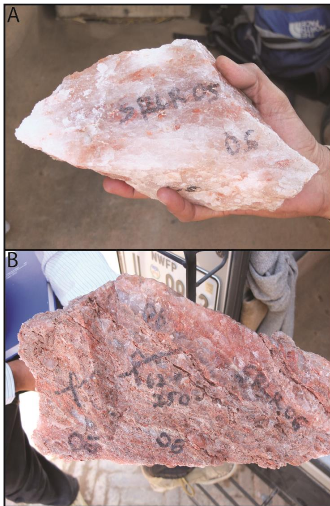
Fig. 3. A) Hand sample SRLR-05 of halite (white) with some bittern salt inclusions (orange) from Khewra Mine. B) Hand sample SRLR-06 of potash marl (red orange) with clear to white crystalline halite from Khewra Mine. For a detailed mineralogical and structural analysis of these samples the reader is directed to Richards et al., 2015.
