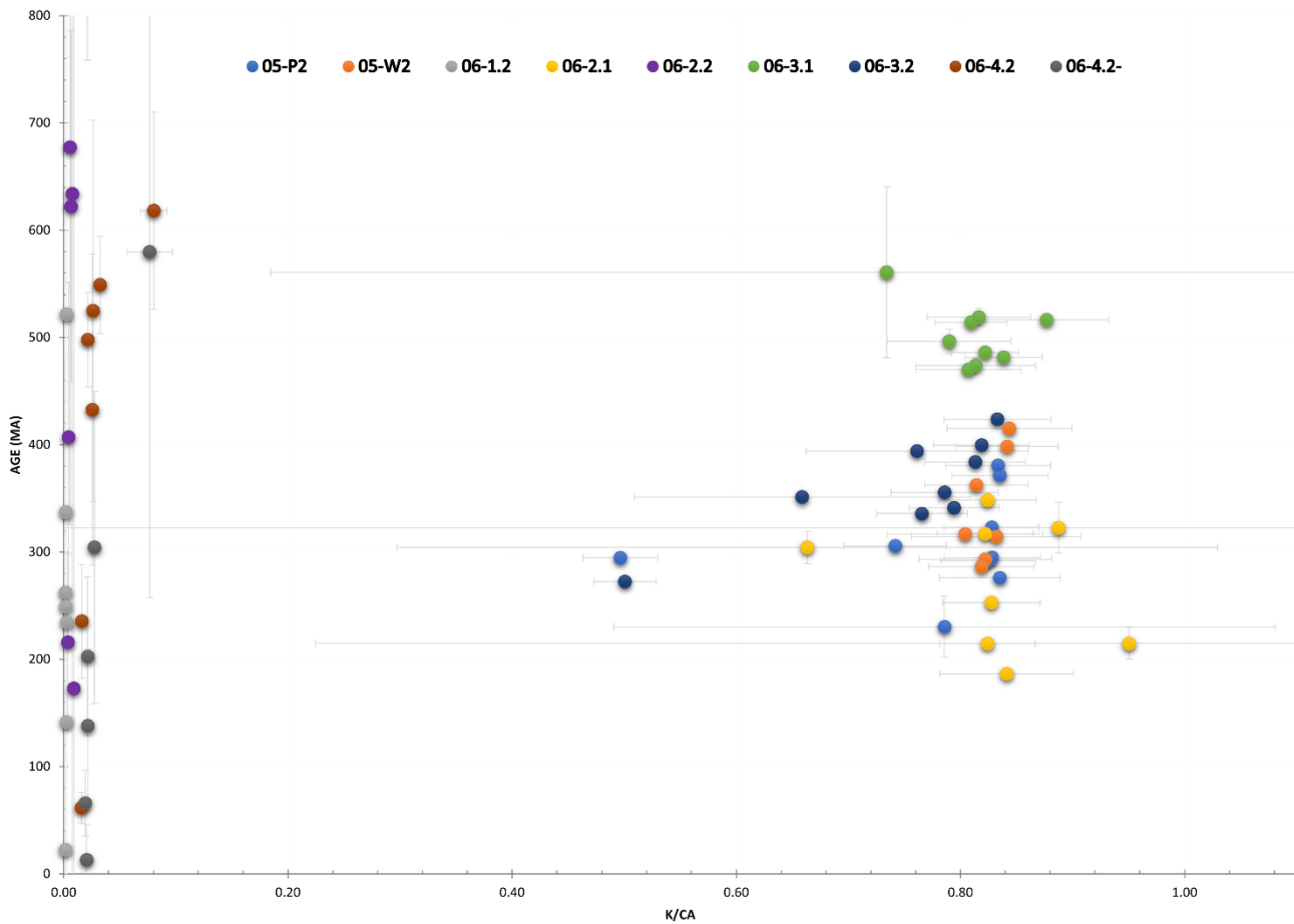
Fig. 4. Measured age vs K/Ca plot displaying two distinct populations within the samples tested.
