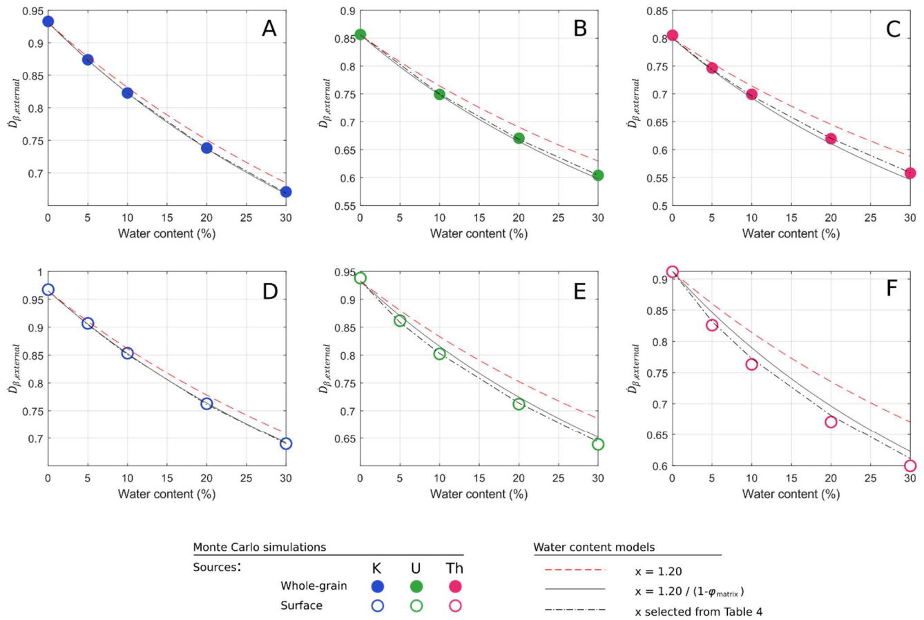
355 Figure 4: Simulated beta dose to 200 \mu\text{m} grains in a sandy matrix (mean grain size 250 \mu\text{m} ), plotted against the water content. Simulations are shown for K, U and Th sources, either whole-grain or surface-held. The external beta dose is expressed as a fraction of the IM beta dose rate. Also shown are predicted dose rates using three different derivation for x .
