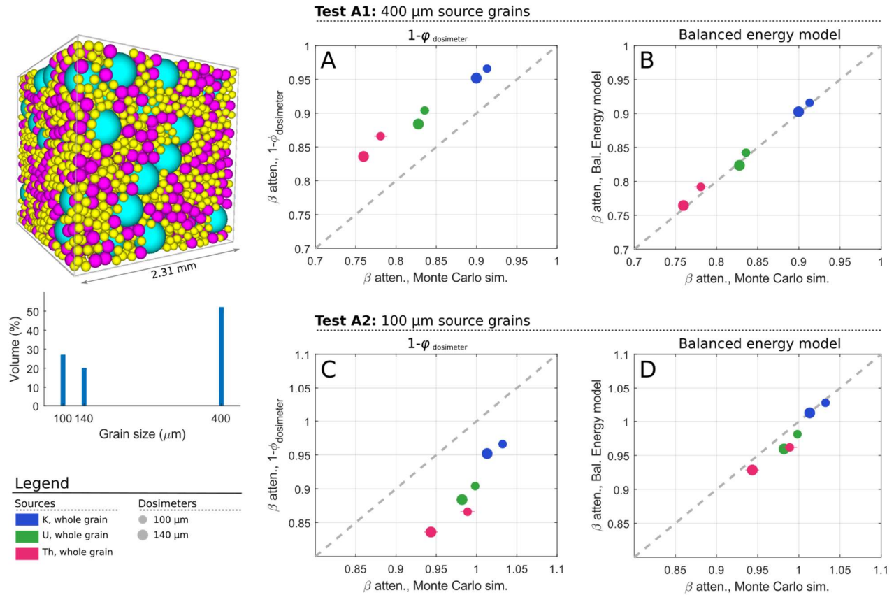
260 Figure 2: Testing beta attenuation models against Monte Carlo radiation transport simulations, using MCNP6 with PackLSD geometry. Geometry configuration A is the geometrical model for two tests, A1 and A2, with an atypical grain-size distribution (colours used in the packing illustration are to help visualise grain sizes). In test A1, the source grains are all 400 \mu\text{m} in diameter, with particles initiated homogenously throughout the grain ('whole grain'), calculated separately for ^{40}\text{K} , U-series and Th-series sources. The mean attenuation factor is shown for 100 \mu\text{m} and 140 \mu\text{m} dosimeters, and compared against (a) 1 - \phi_{dosimeter} (b) balanced energy model. Test A2 shows equivalent results in (c) and (d), when sources are all 100 \mu\text{m} grains.
