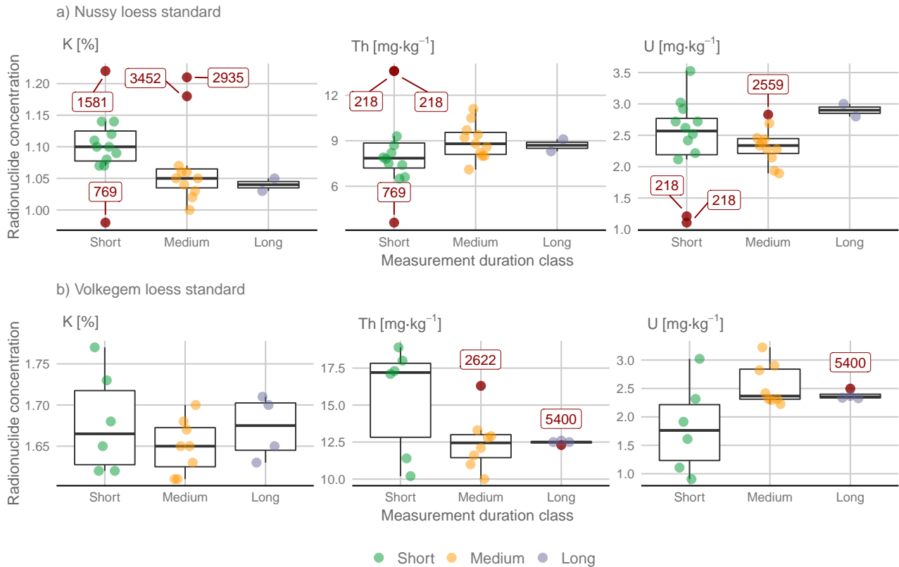
Figure 7. Radionuclide concentrations determined by \mu Dose-measurements given as % for K (left) and as \text{mg} \cdot \text{kg}^{-1} for Th (centre) and U (right). Results of individual measurements and boxplots for the loess standards Nussy (top) and Volkegem (bottom). Data grouped by measurement duration in three classes: short-time ( < 2,000 \alpha -counts; green symbols); medium-time ( 2,000 - 4,000 \alpha -counts; yellow symbols); long-time ( > 4,000 \alpha -counts; grey symbols). Outliers (red symbols) as identified by the 1.5 IQR-criterion and labelled with their respective numbers of total \alpha -counts. Classification not based on specific statistical arguments but reflecting the realisation of the experiments.
