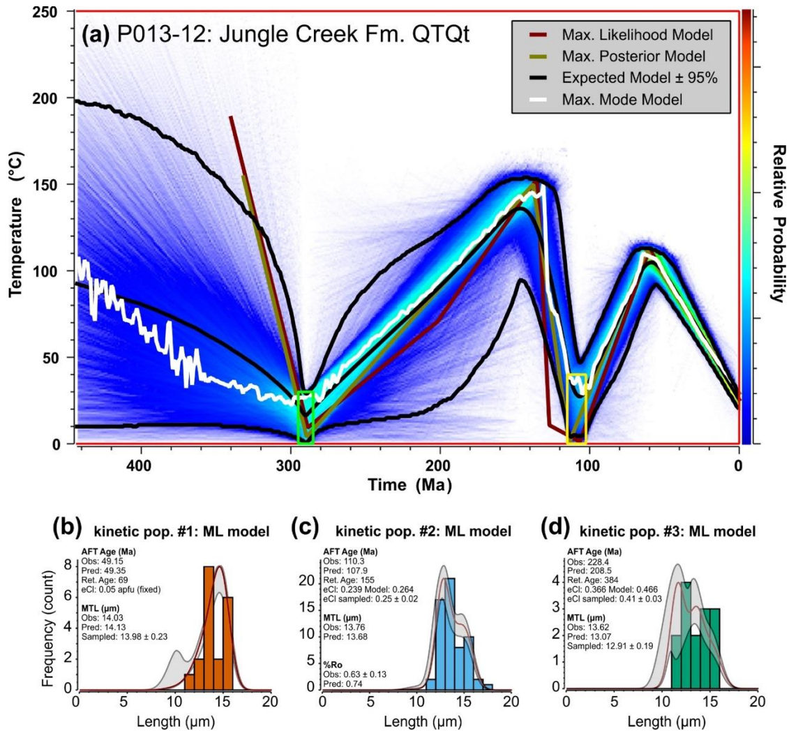
Figure 8: QTQt model results for Permian detrital AFT sample P013-12 (Jungle Creek Formation). (a) Time-temperature plot of the histories retained post burn-in, coloured by relative probability, with warmer colours denoting higher probability. Individual models include the Maximum Likelihood (highest likelihood and best fit; red curve), Max. Posterior (preferred Bayesian model – simplest, balancing fit with complexity; gold curve), Max. Mode (peak of the marginal distribution at 1 m.y. intervals; white curve), Expected (weighted mean of the marginal distribution \pm 95% credible interval; black curves). The latter two models are summaries of the posterior distribution and not directly sampled during the inversion. (b) Max. likelihood fit to the track length distribution and predictions for AFT age and MTL for population one using a fixed eCI value of 0.05 apfu. (c) Max. likelihood fit to the track length distribution and predictions for AFT age and MTL for population two, allowing resampling of the calculated eCI value. (d) Max. likelihood fit to the track length distribution and predictions for AFT age and MTL for population three, allowing resampling of the calculated eCI value. General information: Green box is depositional age of 290 \pm 5 Ma (15 \pm 15 °C). Yellow box is geologic constraint at 108.75 \pm 6.25 Ma (20 \pm 20 °C). Note: All populations utilize the central AFT age in QTQt, whereas the pooled age is used in AFTINV for samples with < 10% age dispersion. Model setup: 500,000 iterations (burn-in) and 500,000 iterations (post burn-in; shown). Prior model space: 300 \pm 300 Ma and 125 \pm 125 °C. Modern surface temperature of 25 \pm 10 °C and maximum allowed \partial T/\partial t of 20 °C/My. Proposal moves were rejected if proposed outside of the prior and more complex models were rejected for equivalent likelihood. See text for further discussion.
