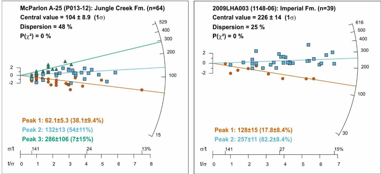
Figure 3: Radial plots of single grain ages for the multikinetik Permian (left) and Devonian (right) AFT samples. Points are colour-coded according to the kinetic populations determined in figure 4 and 5. Peak ages are from age mixture modelling (estimated percentage of grains per population in brackets) and show good correspondence with kinetic population ages summarized in Table 2.
