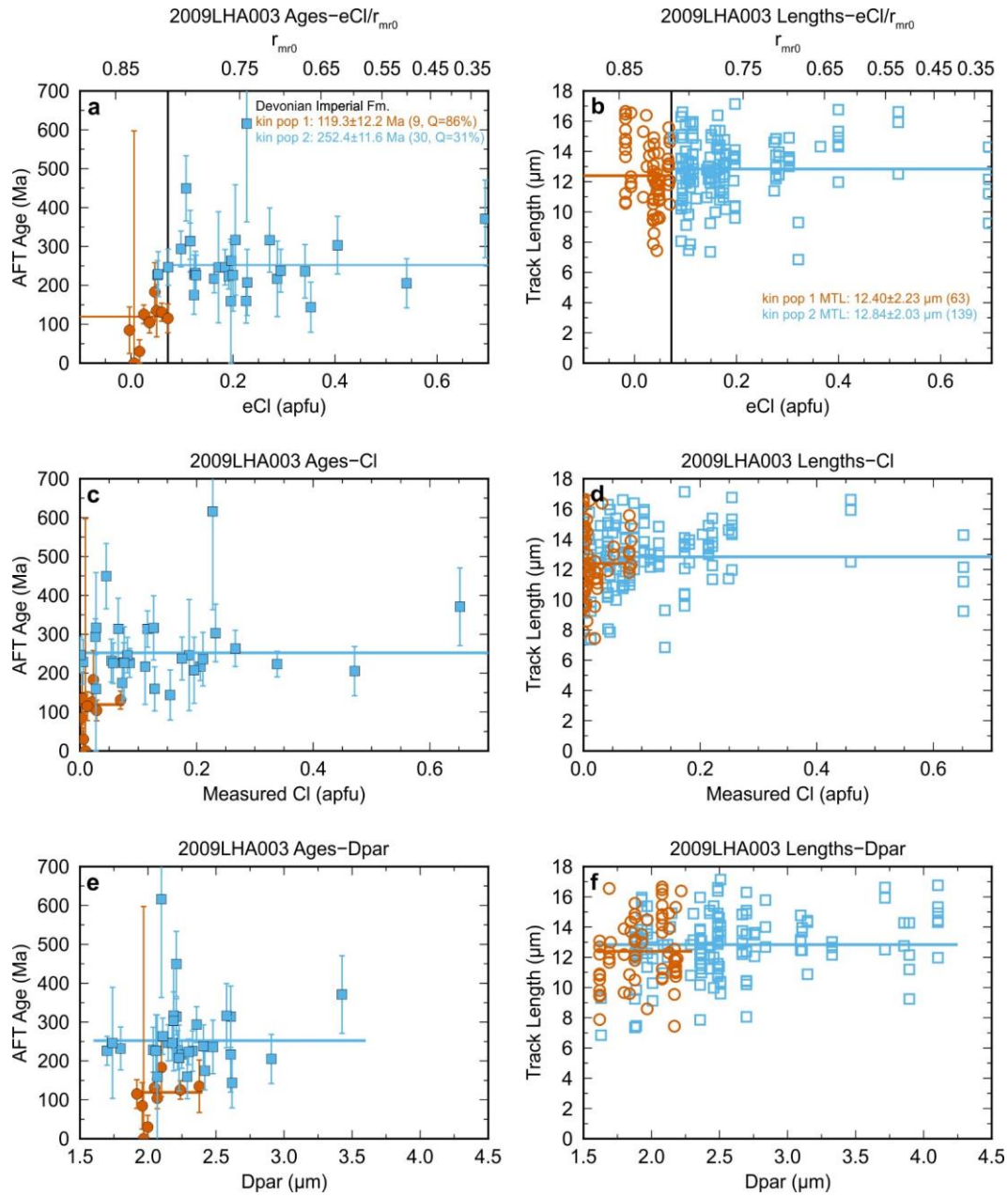
Figure 5: Plots of (a) single grain ages and (b) track lengths grouped into different coloured-coded kinetic populations using eCI values for the Devonian outcrop sample. Boundary between populations is indicated by the vertical black line. Similar plots of population ages and lengths with respect to CI concentration (c and d) and D_{\text{par}} (e and f) with same colour scheme as (a) and (b).
