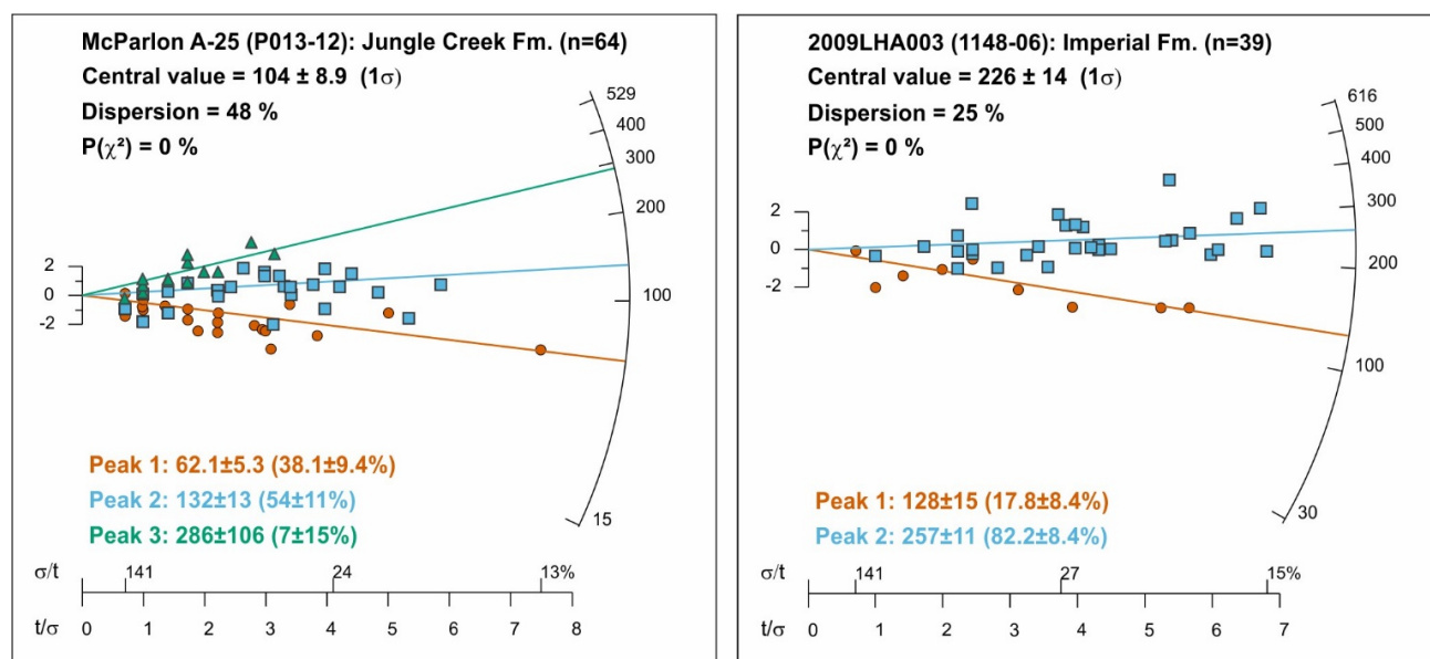
Figure 3: Radial plots of single grain ages for the multikinetik Permian (left) and Devonian (right) AFT samples. Points are colour-coded according to the kinetic populations determined in figure 4 and 5. Peak ages are from age mixture modelling and show good correspondence with kinetic population ages summarized in Table 2.
