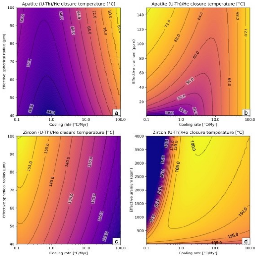
240 Figure 43: Contoured closure temperatures for the apatite and zircon (U-Th)/He systems as functions of cooling rate, effective spherical radius, and eU concentration. (a) Apatite: eU is fixed at 10 ppm; (b) apatite: ESR is fixed at 45 μm; (c) zircon: eU is fixed at 100 ppm; (d) zircon: ESR is fixed at 60 μm. The plots comprise predicted closure temperatures for 20,402 forward models and each model applies a constant cooling rate between 0.1-100 °C/Myr.
