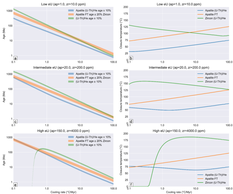
Figure 54: Predicted thermochronometer ages (left) and closure/annealing temperatures (right) for low (top), intermediate (middle), and high (bottom) eU concentrations, as a function of cooling rate. The plots comprise predicted ages and closure temperatures for 303 forward models and each model applies a constant cooling rates between 0.1-100 °C/Myr. The coloured swaths for the predicted ages (a, c, e) indicate the mean age plus or minus the indicated percent uncertainty.
