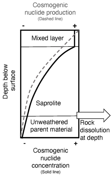
580 Figure 1: Conceptual diagram showing cosmogenic nuclide production and concentration in a column of soil, saprolite, and rock. The dashed line shows decreasing production of cosmogenic nuclides with depth; solid line shows nuclide concentration with depth, and the white arrow represents mass loss by solution below the depth of significant cosmogenic nuclide production.
