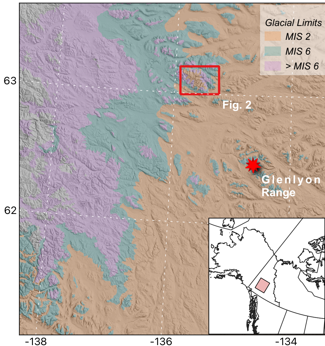
55 Figure 1. Map of the Grey Hunter Region delineating the Grey Hunter massif (red box) as shown in Figure 2 and former CIS glacial limits (shading) . Also shown is the Glenlyon Range.
