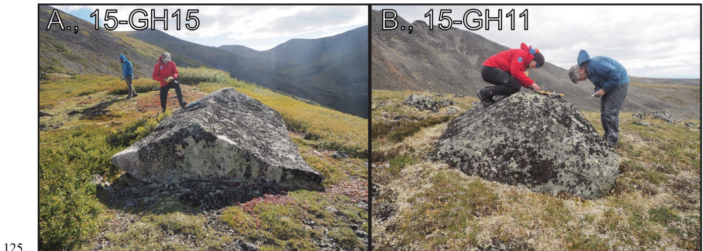
Figure 3. Example of boulders sampled from outer moraines (15-GH15; A.) and inner moraines (15-GH11; B.). Note in A. the embedded character of the far-side of the large erratic.
