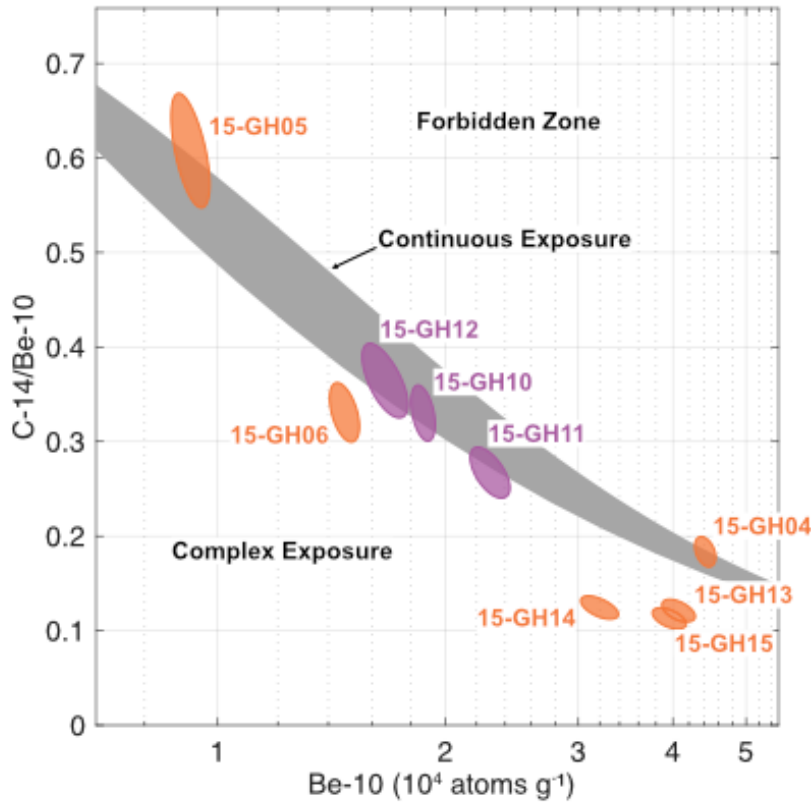
170 Figure 6. Paired ^{14}\text{C} - ^{10}\text{Be} plot demonstrating that two outer moraine samples, GH05 and GH04, are consistent with a single-stage continuous exposure history with little or no surface erosion (upper bound of gray shaded region), the three inner moraines samples are consistent with continuous exposure but also could be affected by a multi-stage exposure history with ^{10}\text{Be} inheritance, and finally four samples from the outer moraines are consistent with complex multi-stage exposure history. Note that ^{10}\text{Be} inheritance serves to lower the ^{14}\text{C} - ^{10}\text{Be} ratio and shift samples to the right. Outer (inner) moraine samples are shown in orange (purple).
