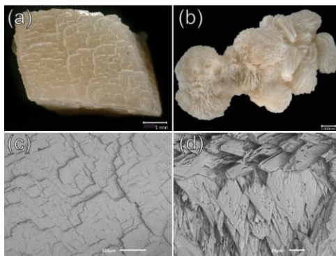
Figure 1: Selected CCC morphologies of patch 1. (a) Rhombohedral calcite crystal with stepped surface, (b) complex intergrown crystals composed of radial-fibrous calcite, (c) SEM image of the surface of the sample depicted in (a), (d) SEM image of (b).
