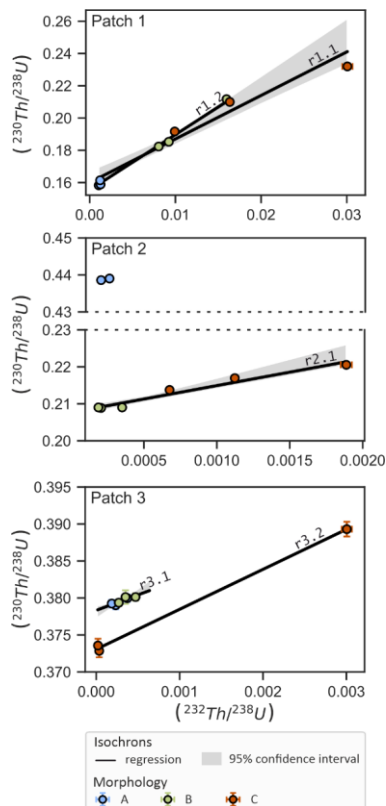
Figure 4: Isochron plots of ^{238}\text{U} -normalised thorium measurements of each CCC patch. Colour represents morphological type. The shaded area represents the 95% confidence interval of the regression slope and intercept. Regression lines are labelled with an identification number corresponding to supplementary table 1.
