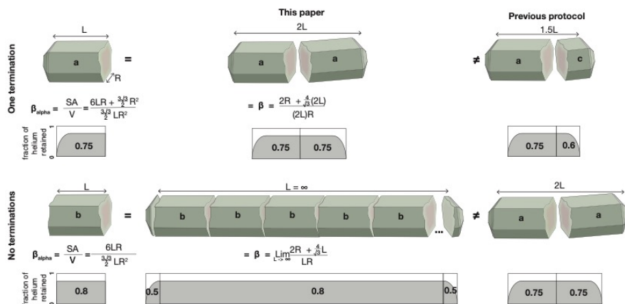
175 Fig. 1. The alpha-ejection-affected surface-area-to-volume ratio, or \beta_{\alpha} , of a broken crystal that has lost a basal fragment longer than one alpha-stopping distance is equivalent to the surface-area-to-volume ratio of an unbroken crystal twice as long (for fragments with one termination), and equivalent to that of an unbroken crystal infinitely long (for fragments with no termination). The simple geometric calculations shown assume a flat hexagonal termination, but apply by the same logic to any geometry, regardless of the 180 shape of its body (e.g. cylindrical, tetragonal, or hexagonal) or the shape of its terminations (e.g. pyramidal, flat, or rounded). The profiles of fraction of helium retained that are shown below each fragment are schematic and serve only to illustrate the equivalence or non-equivalence of fragments of different lengths (e.g. a = 0.75, b = 0.8, c = 0.75), and do not correspond to any specific dimensions. As discussed in text, these calculations assume no change to the daughter concentration profile due to diffusion.
