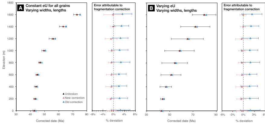
350 Fig. 6. a) Date-elevation transect of a crustal block that cooled slowly through the partially retention zone, and was subsequently rapidly exhumed (cf. Brown et al. 2013, Fig. 9), showing fragment dates corrected using the new protocol (red), compared to previous protocol (blue), and the expected whole-crystal date (black). Note that the red and black triangles may be difficult to distinguish because they overlap in most cases. Corrected dates are from fragments of varying lengths, both singly and doubly broken, generated from crystals with variable widths and lengths, but constant eU. Error bars in date-elevation transect represent intra-sample date dispersion and are shown for the new protocol only. Error bars in the right panel show the % deviation of the corrected fragment dates from their corresponding corrected whole-crystal dates, using the new (red) and old protocol (blue). (b) Same as (a), but fragments were generated from crystals of varying eU (15-100 ppm, Brown et al., 2013), in addition to varying width and length. Notice that the introduction of eU as a variable significantly increased the intra-sample dispersion of corrected dates, but that the error attributable to the fragmentation correction alone was not materially affected. All error bars are 1\sigma .
