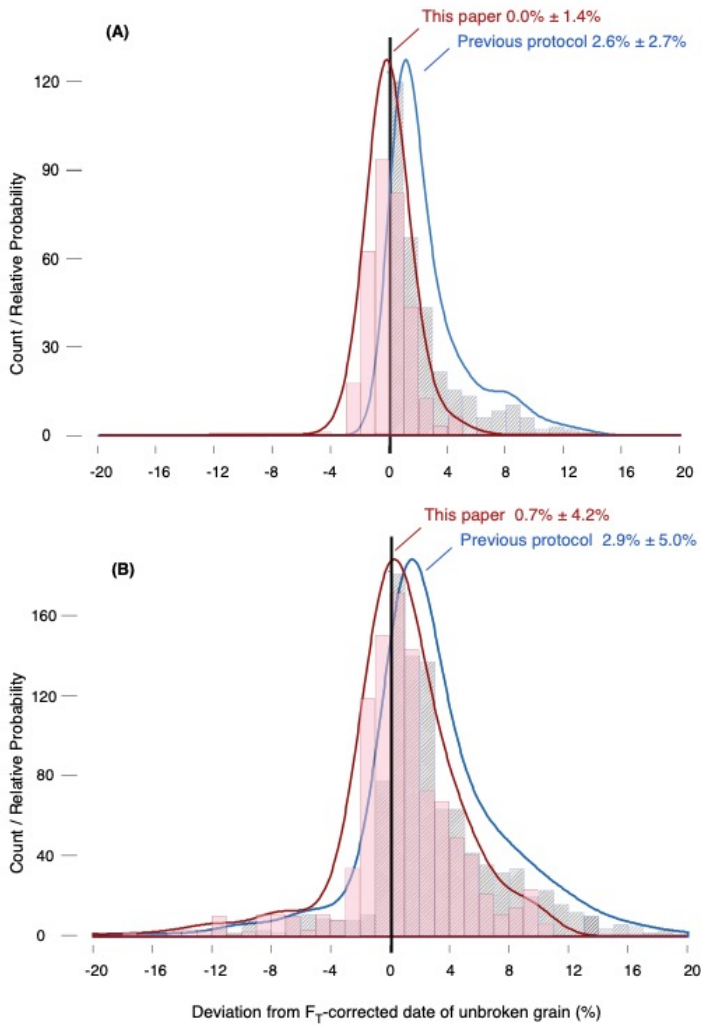
Fig. 2. Histograms and kernel density estimate (KDE) functions comparing the new protocol suggested in this paper (red) and the previous protocol (blue), as applied to a synthetic dataset of raw, uncorrected dates ( n=1000 , cf. Brown et al., 2013). The error is defined to be the % deviation of the F_T -corrected dates of a broken crystal from the F_T -corrected date of the whole crystal, which is known because the synthetic fragments are generated from a whole crystal with a known “age”. The new protocol is more accurate and more precise at correcting for the effect of fragmentation, both in the ideal case (A) assuming that fragmentation has occurred more than one average-alpha-stopping-distance from the tip, and that there is no significant diffusive modification of the helium profile, as well as in the more realistic scenario (B) when these assumptions are relaxed. In other words, (B) includes corrected dates from fragments that are broken close to the tip, and fragments that experienced thermal histories leading to significant diffusive modification, in addition to the dates contained in (A). Annotations show the mean \pm standard deviation ( 1\sigma ); KDE functions are normalized to the same peak height.
