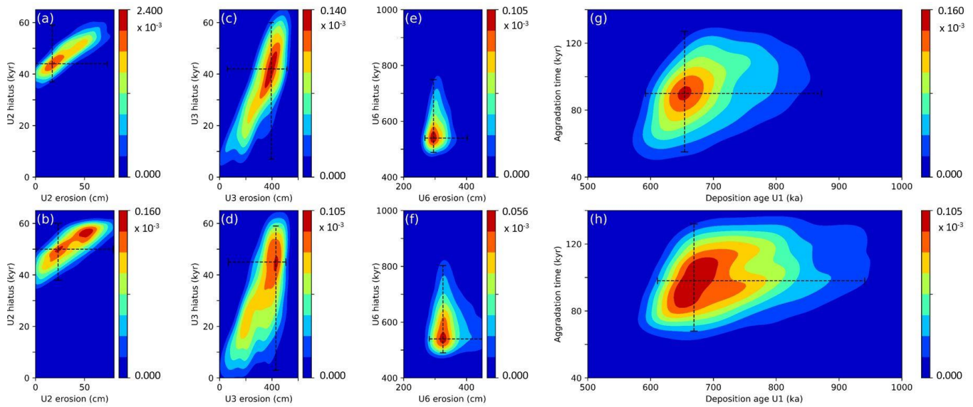
410 Figure 7: Density plot of the possible model outcomes for scenario 4. Any simulation that returned a reduced 411 chi-squared smaller than 1.83 is considered to be significant, and included as a possible solution in the 412 density plots. The density of significant solutions is shown by color coding. The four upper panels (a, c, e, g) 413 represent the parameters of simulations (n=486) characterized by a 26 Al/ 10 Be of 6.75, and the lower panels 414 (b, d, f, h) the parameters of simulations (n= 1695) with a 26 Al/ 10 Be of 7.40. For each parameter, the most 415 likely value (i.e. value with highest density of significant solutions) is reported as well as its 95% confidence 416 interval (2σ). The 95% confidence interval is derived from the 2.5 % and 97.5 % limits of the kernel 417 cumulative density function.
