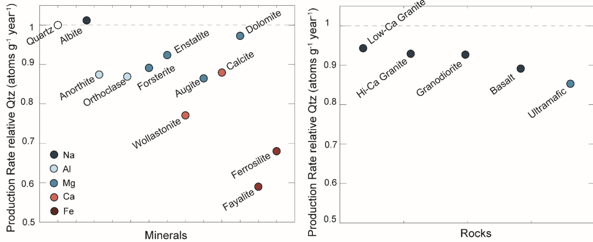
Figure 3: SLHL production of minerals (left) and rocks (right) compared to quartz (dashed grey line). The minerals and rocks are colored for what element contributes the highest proportion of production after oxygen and silica.
