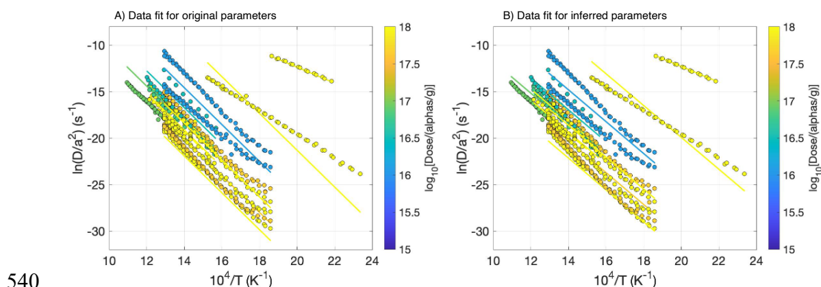
Figure 1. Key parameters controlling how radiation damage controls diffusivity have been inferred from fitting Arrhenius relationships from step-degassing experiments. A) The fit to the step-degassing experiments for the model parameters inferred by Guenther et al., (2013). B) The fit to the step-degassing experiments using model parameters extracted from the data using a Markov Chain Monte Carlo analysis. The model parameters are the minimum misfit model parameters and represent a single realization of the parameter set we infer. The point of this figure is not to show that one model predicts the diffusion data better than the other. It is simply to show the fits to the data and the data that are used to predict the model parameters, and to highlight that both models do not predict all the data.
