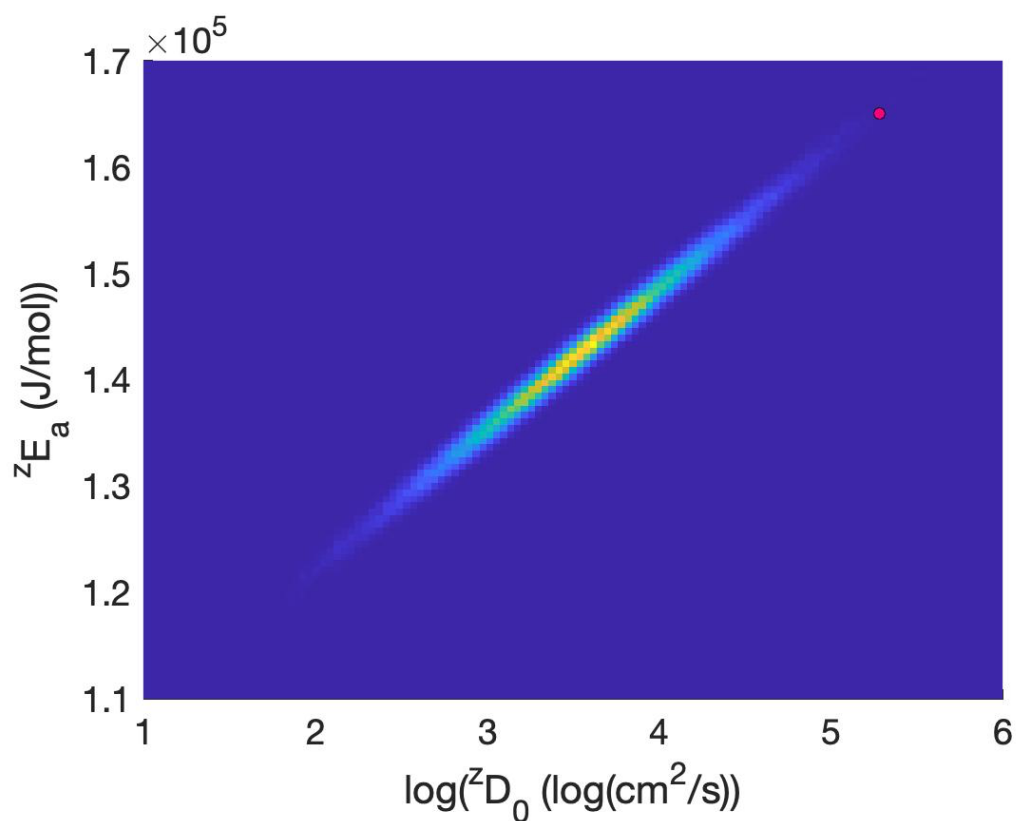
560 Figure 3. Inferred model parameters from diffusion data are strongly correlated. Our approach to infer the diffusion kinetics of the hypothetical crystals using the radiation damage model maintains this correlation. This is clearly illustrated with the diffusion parameters for the undamaged crystal. The pink spot shows the diffusion kinetics inferred by Guenther et al., (2013) and while it is reasonably far from the center of our inferred distribution, it still falls on the clear correlation trend defined by the sampling. The colours are 565 proportional to posterior probability with oranges/yellows reflecting highest probabilities.
