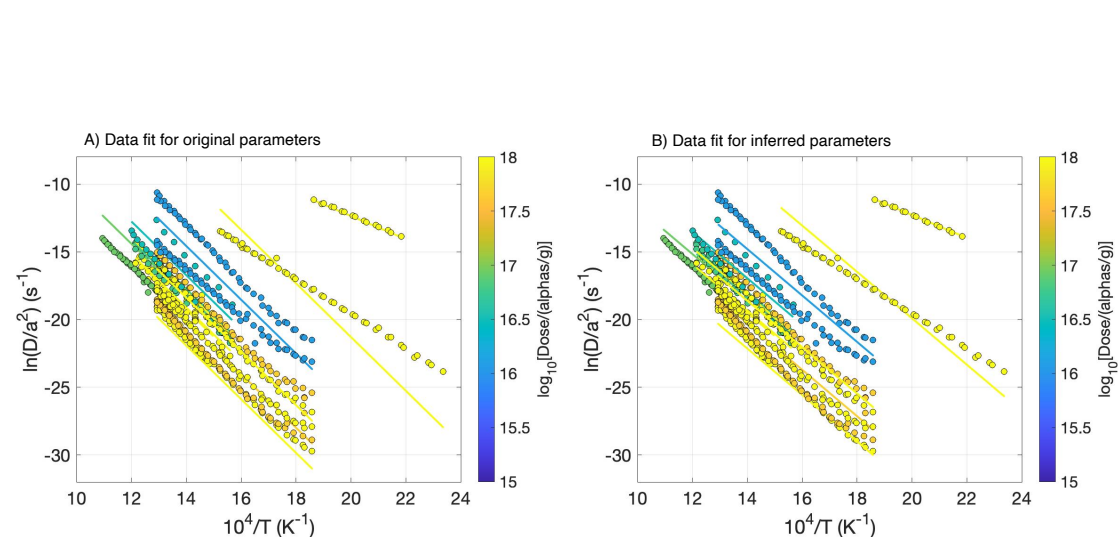
Figure 1. Key parameters controlling how radiation damage controls diffusivity have been inferred from 620 fitting Arrhenius relationships from step-degassing experiments. The datapoints are shown by circles and the lines represent model fit. Both are coloured by the alpha dose. A) The fit to the step-degassing experi- ments for the model parameters inferred by Guenther et al., (2013). B) The fit to the step-degassing experi- ments using model parameters extracted from the data using a Markov Chain Monte Carlo analysis. The
