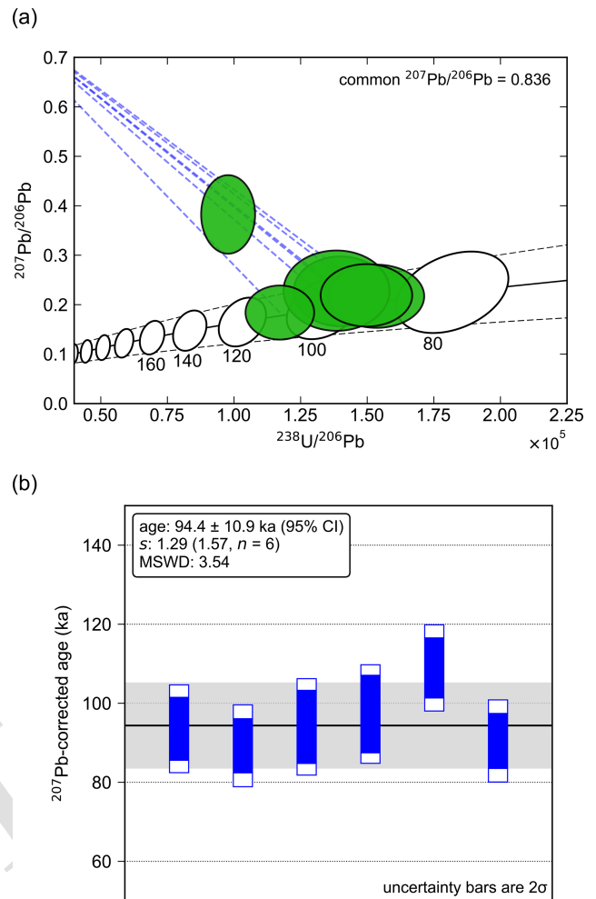
Figure 5. Example of ^{207}\text{Pb} -corrected age plots. (a) Data ellipses plotted on a Tera–Wasserburg diagram as 95 % confidence ellipses (green). The black line shows the disequilibrium concordia constructed using D_{\text{Th}/\text{U}} = 0.2 \pm 0.03 (TS2) ( 2\sigma ) and D_{\text{Pa}/\text{U}} = 2.9 \pm 1.0 ( 2\sigma ), with dashed black lines indicating uncertainty bounds (95 % CI). Concordia markers are plotted as 95 % age ellipses, representing x – y uncertainty for a given age due to uncertainty in distribution coefficients. The dashed blue lines show a line projecting from the common Pb point at the y intercept ( ^{207}\text{Pb}/^{206}\text{Pb} = 0.836 ) through the centre of each data point to its intercept with the disequilibrium concordia. (b) Plot of individual ^{207}\text{Pb} -corrected ages. The dark blue bars indicate age uncertainties ( 2\sigma ) accounting for random analytical uncertainties only, while the larger white bars show combined random and systematic uncertainties ( 2\sigma ) (i.e. including components due to uncertainty in D_{\text{Th}/\text{U}} and D_{\text{Pa}/\text{U}} values). The black line shows the weighted average age computed using the robust spine algorithm which accounts for the age covariance structure, with the light grey shading indicating a 95 % confidence interval on this weighted average. Initial disequilibrium corrections were applied assuming constant distribution coefficient ratios, i.e. approach (i) in Sect. 3.1, treating uncertainties in D_{\text{Th}/\text{U}} and D_{\text{Pa}/\text{U}} as purely systematic uncertainties.
