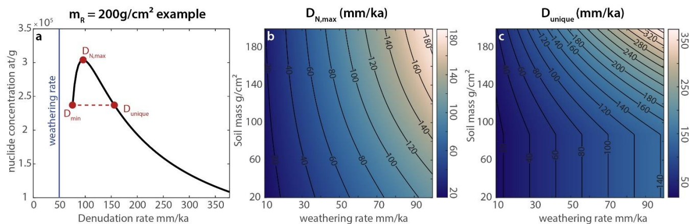
Fig. 7. Weathering impact on the nuclide concentration of 36 Cl measured in pure calcite at SLHL. C_{aB} = 0.7 , Q_B = 0.3 , m_R = 200 g/cm 2 . (a) 36 Cl concentration versus denudation rate for calcite. The nuclide concentration increases above D_{min} until D_{N,max} . At denudation rates higher than D_{unique} , 36 Cl measurements would be unambiguous. (b) D_{N,max} for the same sample, and a range of weathering rates and regolith masses. (c) same as (b) for D_{unique} .
